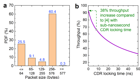
Fig. 1: (a) Packet size distribution and (b) Throughput against CDR locking time
