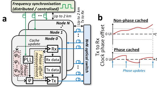
Fig. 2: (a) Synchronised optically switched data centre architecture, (b) Operational principle of phase caching.
