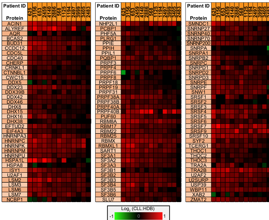
B. All quantified spliceosome components
