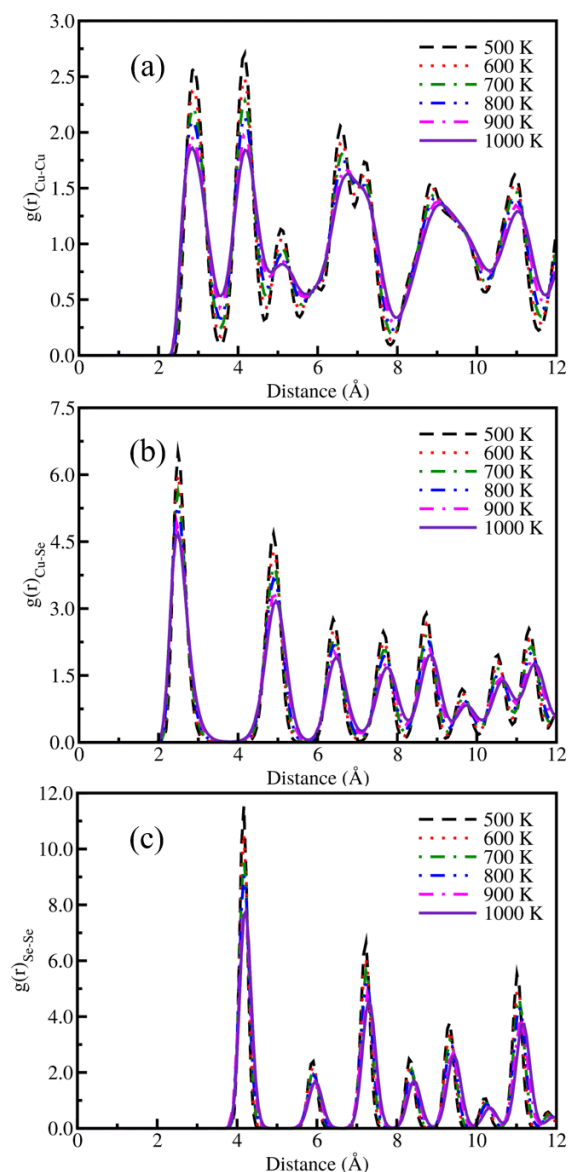
Figure 6. The RDF at different temperatures for (a) Cu-Cu (b) Cu-Se and (c) Se-Se pairs.
