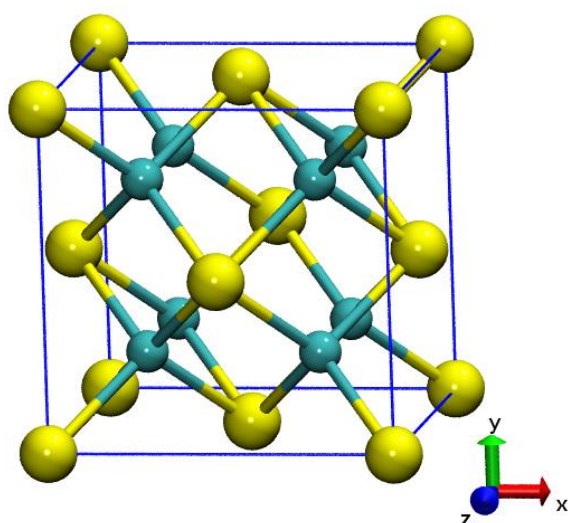
Figure 1. The FCC unit cell of \beta -Cu 2 Se; yellow (Se) and cyan (Cu)
