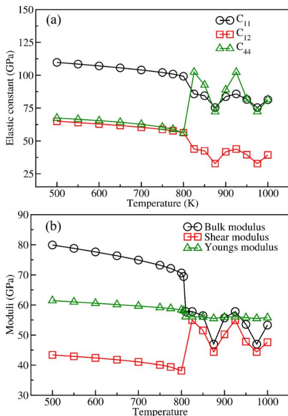
Figure 5. (a) Change in elastic constants with temperature (b) Change in bulk, shear and Young's modulus with the temperature.
