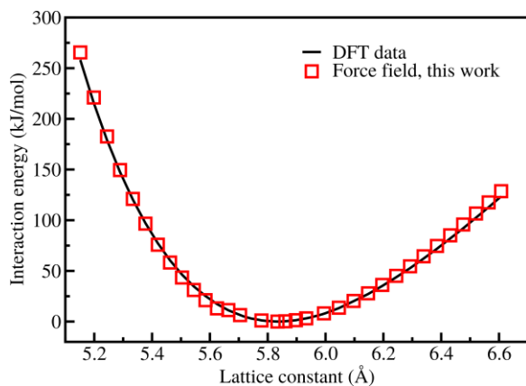
Figure 3. A comparison of energy-volume data obtained from DFT and the new empirical force-field
