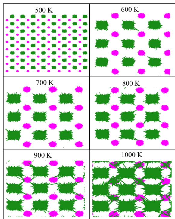
Figure 8. The atomic trajectories, unwrapped coordinates, of atoms in XY-plane at different temperatures. The Cu and Se atom trajectories are shown in green and pink color, respectively.
