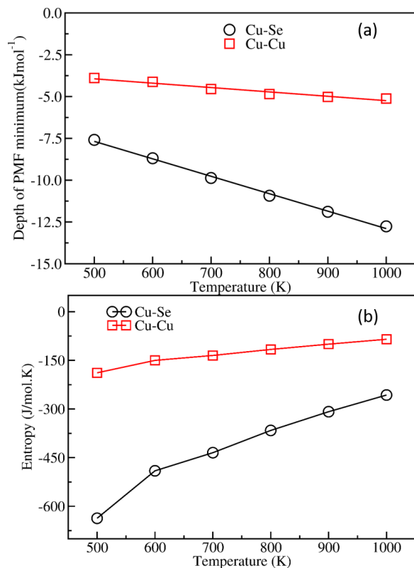
Figure 10. (a) The free energy of aggregation for Cu-Cu and Cu-Se atoms is shown at different temperatures; solid line shows the straight line fit to the simulation data (b) The excess entropy associated with the Cu-Cu and Cu-Se interactions is presented at different temperatures.
