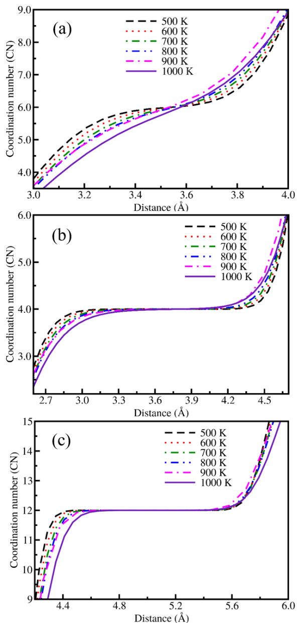
Figure 7. Coordination number for (a) Cu-Cu (b) Cu-Se and (c) Se-Se at different temperatures.
