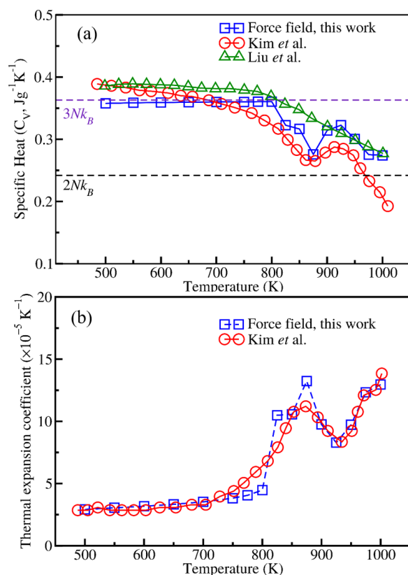
Figure 4. (a) Comparison of heat capacity data obtained using the generated force-field with the experimental data. (b) Comparison of CTE obtained using the generated force-field with the experimental data.
