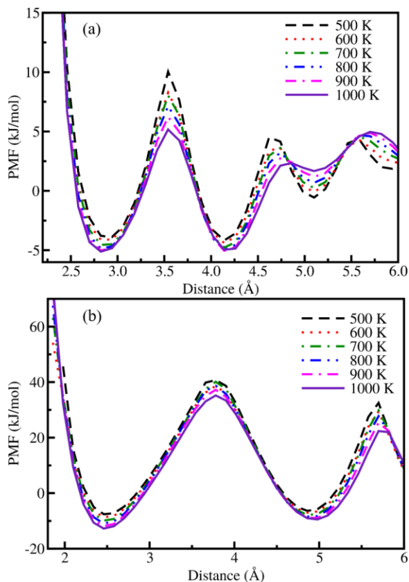
Figure 9. The PMF calculated at different temperatures using (a) Cu-Cu and (b) Cu-Se RDF data.
