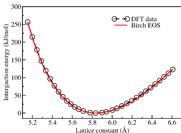
Figure 2. Energy-volume data generated using DFT for \beta -Cu 2 Se structure. The solid red curve represents the fit to the Birch-EOS.
