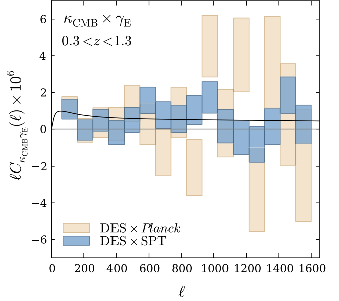
Figure 2. \kappa_{\text{CMB}}\gamma_E correlation measured in harmonic space with POLSPICE . Projected angular power spectra, C(\ell) , are shown for DES \times SPT (blue boxes) and DES \times Planck (orange boxes). Sources come from the ngmix shape catalogue and span the redshift range 0.3 < z < 1.3 , selected using the SkyNet2 photo- z catalogue. The height of the bars represents 68 per cent error limits. The theoretical prediction for the cross-correlation, with amplitude A = 1 , is also shown (black solid line).
