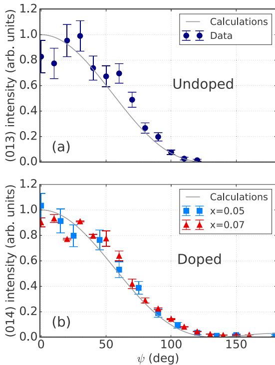
FIG. 7. Azimuthal dependence [azimuthal reference (010)] of the (013) and (014) magnetic diffraction peaks in the (a) undoped and (b) doped ( x = 0.05, 0.07 ) samples at T = 7-8 K, respectively. The filled symbols refer to the scattered intensity integrated over a rocking curve at E = 2.838 keV corrected for the geometry-dependent self-absorption factor [30]. The solid lines represent the calculated azimuthal dependence (except for an arbitrary scale factor) assuming the C-AFM structure with \mathbf{b} -axis moments reported by Braden et al. [19]. The intensity is normalized to the calculated value at \psi = 0^\circ .
