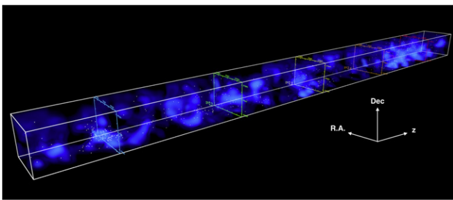
Figure 10. Still image from our 3D video visualization of the CLAMATO reconstructed absorption map (smoothed with a R = 2 h^{-1} Mpc Gaussian kernel), where the absorption is indicated by the blue transparency. Foreground galaxy redshift positions are denoted by the yellow dots, while the triad (not present in the video) indicates the directions of increasing R.A., declination, and redshift. Alternatively, the YouTube version ( https://youtu.be/QGXi7P4u4g ) offers a virtual-reality option when viewed with a smartphone and a headset compatible with Google Cardboard.
