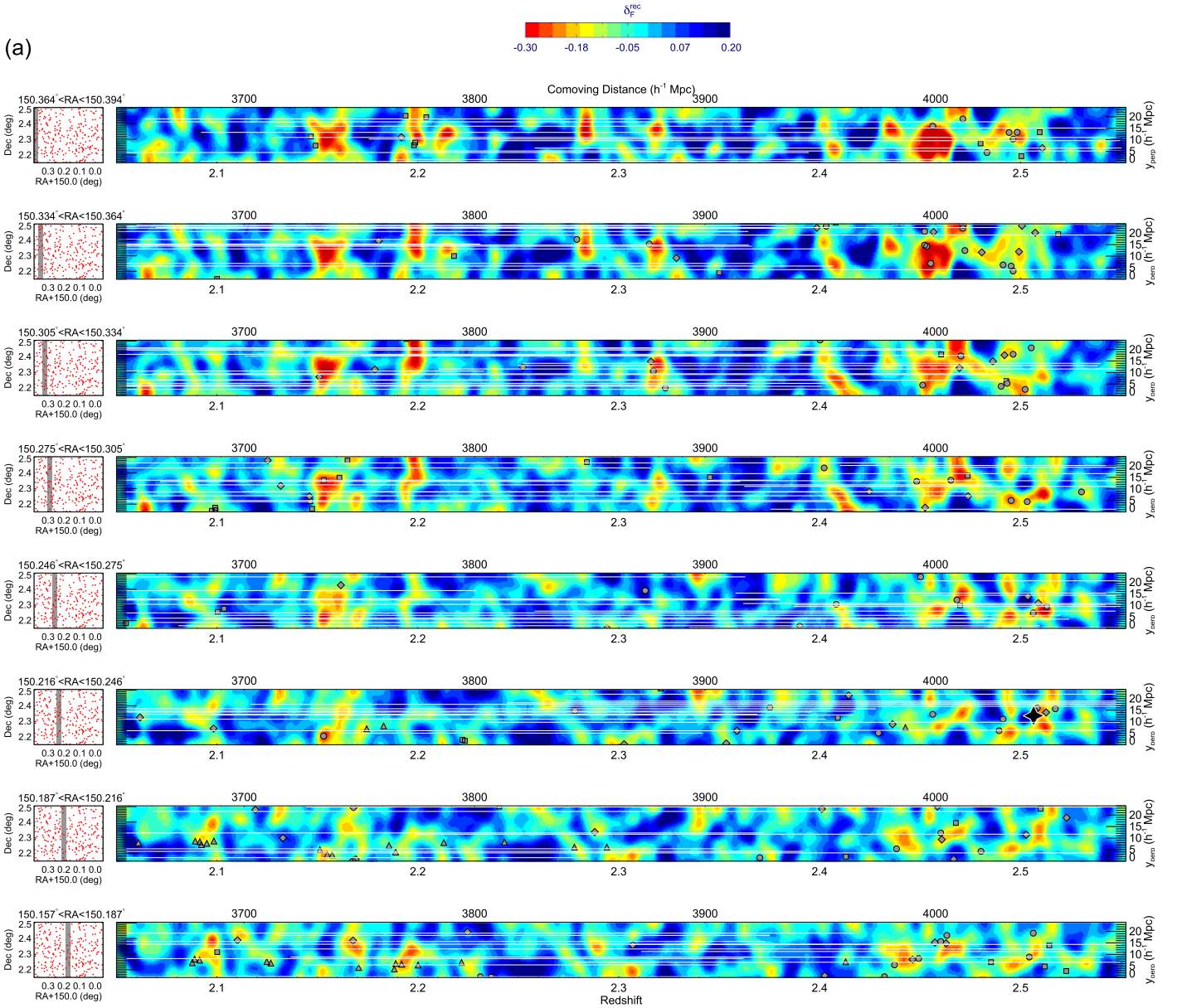
Figure 9. Wiener-filtered tomographic reconstructions of the Ly \alpha forest absorption field, \delta_F^{\text{rec}} , at 2.05 < z_\alpha < 2.55 from the current CLAMATO data (color map), shown after smoothing with an isotropic R = 2 h^{-1} Mpc Gaussian kernel. Each color panel shows the absorption projected over a 2 h^{-1} Mpc R.A. slice, the position of which is denoted by the shaded region in the subpanels to the left that also show the sightline positions on the sky as red dots. The color convention for the absorption is such that red denotes overdensities, while blue denotes underdensities. White horizontal lines denote the sightline coverage, while symbols mark the location of known foreground galaxy redshifts: downward triangles for MOSDEF, upward triangles for ZFIRE, squares for VUDS, diamonds for zCOSMOS-Deep, and circles for CLAMATO. The large black stars indicate the reported central positions of the galaxy overdensities at z = [2.10, 2.44, 2.47, 2.51] . This sequence is continued in Figure 9(b).
