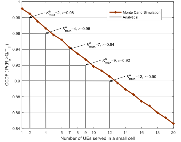
Fig. 2. The complementary cumulative distribution function (CCDF) of the R_a : \frac{Q}{T_{\text{th}}} = 1 Mbps, \lambda_U = 3 \times 10^{-4} \text{ m}^{-2} , \lambda_S = 10^{-4} \text{ m}^{-2} , \eta = 0.5 , and Cache Size = 3 \times 10^3 .
