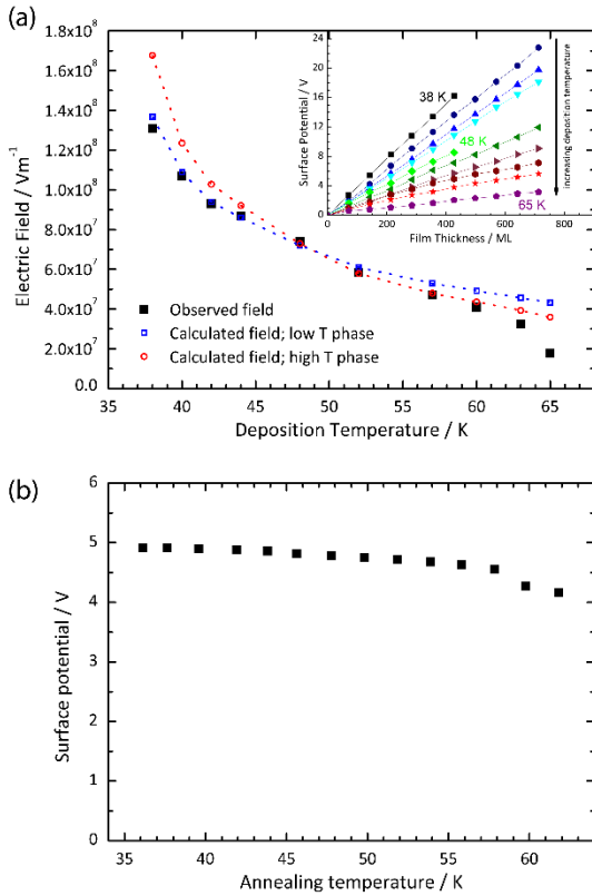
Figure 4. a) The electric field measured in films of N 2 O plotted as a function of film deposition temperature (black squares), with the calculated fields for the low temperature (blue squared) and high temperature phase (red circles) superimposed. The lines act as a guide to the eye. The inset shows how surface potentials develop as a function of film thickness across a range of film deposition temperatures (38-65 K). b) Surface potential of a film of N 2 O deposited at 38 K and annealed in steps up to 62 K. At each temperature time was given to reach thermal equilibrium and then the surface potential at the film-vacuum interface was measured.
