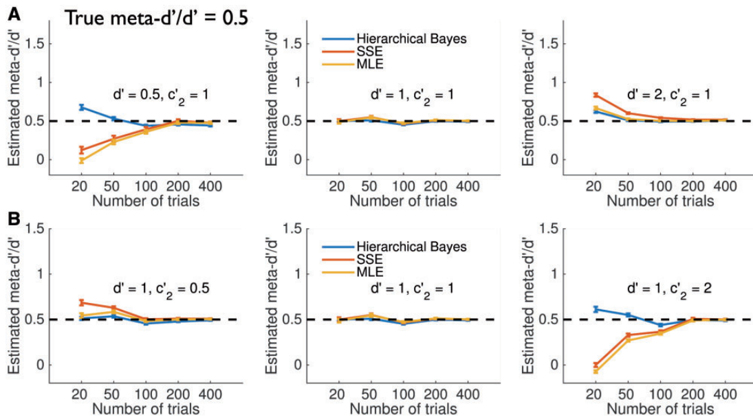
Figure 6. Simulation experiments—low metacognitive efficiency ( \text{meta-}d'/d' = 0.5 ). For legend see Fig. 5.
