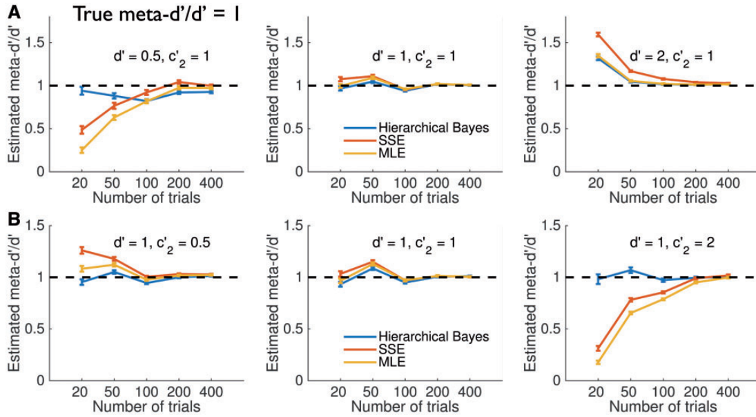
Figure 5. Simulation experiments—medium metacognitive efficiency ( \text{meta-}d'/d' = 1 ). (A and B) Estimated \text{meta-}d'/d' ratio for different fitting procedures while varying (A) d' values or (B) type 2 criteria placements. Each data point reflects the average of 100 simulations each with N = 20 subjects. Error bars reflect standard errors of the mean. The ground truth value of \text{meta-}d'/d' is shown by the dotted line.
