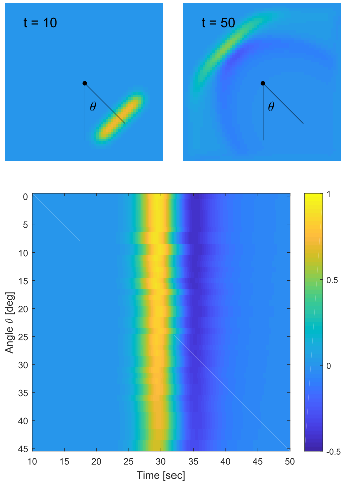
Fig. 2. A rotating on-grid line source emitting a Gaussian pulse. (Top) Snapshots of the acoustic field for \theta = 45^\circ . The acoustic sensor is indicated by a black disc. (Bottom) Magnitude of the acoustic field at the sensor over time as a function of the source's orientation angle \theta . Staircasing errors are evident in the amplitude variations and time-offsets in the sensor data.
