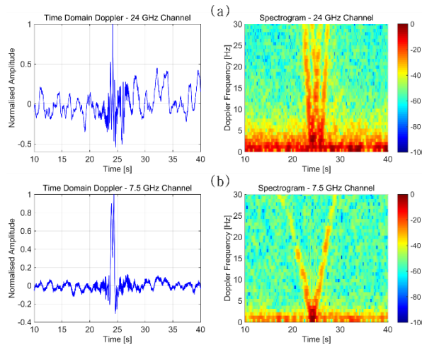
Figure 16 FSR experimental data for third experiment described. (a) and (b) show time domain Doppler and corresponding spectrograms for 24 and 7.5 GHz radar channels respectively
