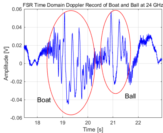
Figure 19 Zoomed FSR time domain Doppler signature of boat towing the ball. Targets are separated due to the difference in the FSR baseline crossing times.
