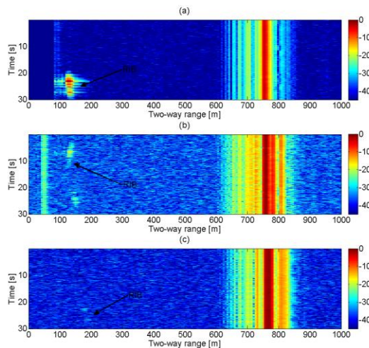
Figure 10 Range-Time plots of the second joint experiment as recorded at NetRAD node 3 (a), node 1 (b), and node 2 (c)
