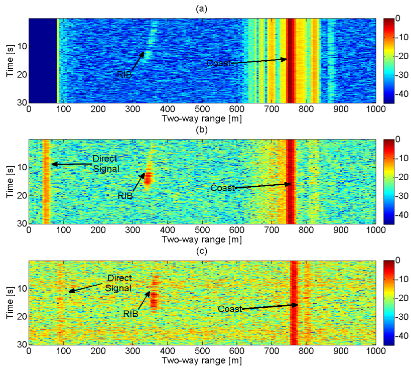
Figure 6 Range-Time plots of the first joint experiment as recorded at NetRAD node 3 (a), node 1 (b), and node 2 (c)
