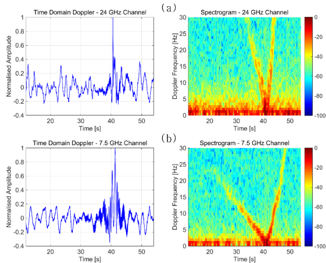
Figure 8 FSR target data for experiment 1. (a) and (b) show time domain Doppler and corresponding spectrograms for 24 and 7.5 GHz radar channels respectively.
