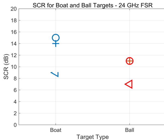
Figure 21 Comparison of SCR's for the FSR 24 GHz measurements of boat and ball target. Similar markers indicate measurement from a single data record of the boat towing the ball.
