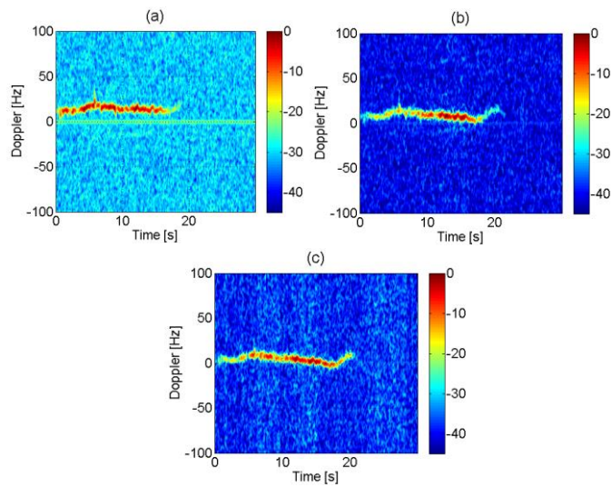
Figure 7 Time-Doppler plots of the 1st joint experiment as recorded at NetRAD node 3 (a), node 1 (b), and node 2 (c)
