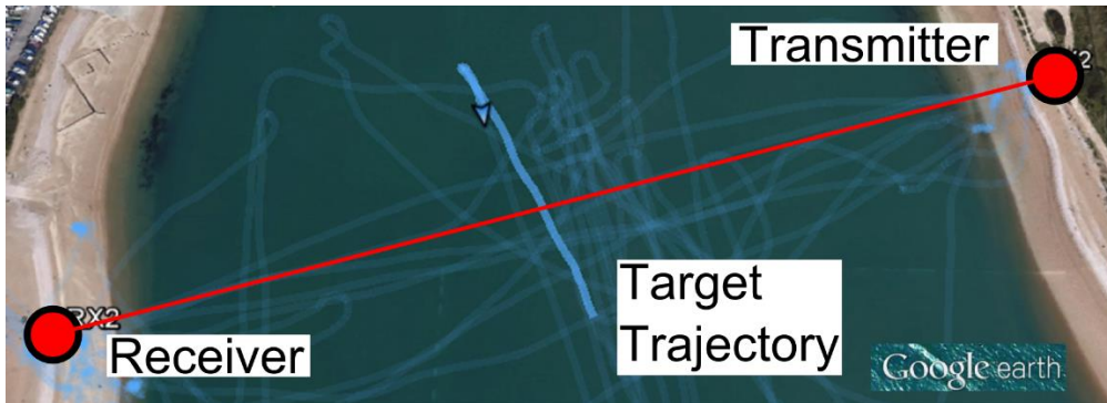
Figure 5 GPS track showing target trajectory for first described experimental data.
