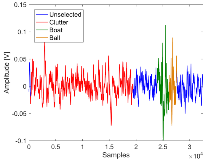
Figure 20 FSR time domain Doppler signature highlighting selected parts of signal for analysis: clutter, boat and ball targets.
