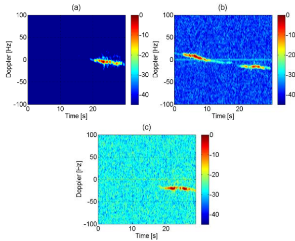
Figure 11 Time-Doppler plots of the second joint experiment as recorded at NetRAD node 3 (a), node 1 (b), and node 2 (c)
