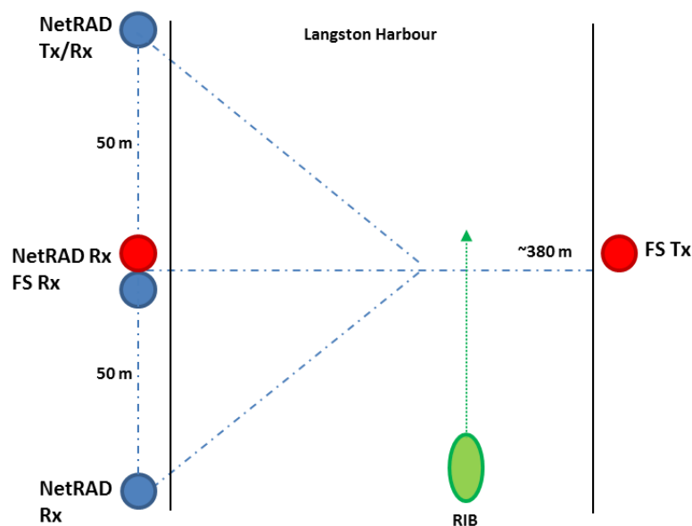
Figure 1 Diagram of experimental setup
