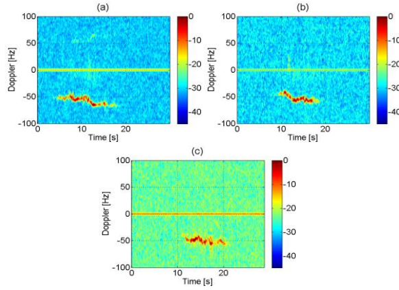
Figure 15 Time-Doppler plots of the third joint experiment as recorded at NetRAD node 3 (a), node 1 (b), and node 2 (c)
