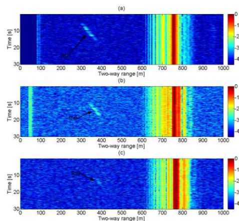
Figure 14 Range-Time plots of the third joint experiment as recorded at NetRAD node 3 (a), node 1 (b), and node 2 (c)
