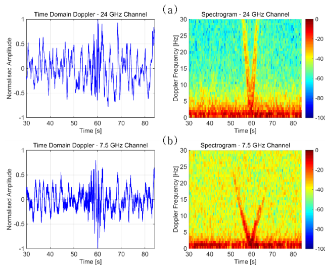
Figure 12 FSR experimental data for experiment 2. (a) and (b) show time domain Doppler and corresponding spectrograms for 24 and 7.5 GHz radar channels respectively.
