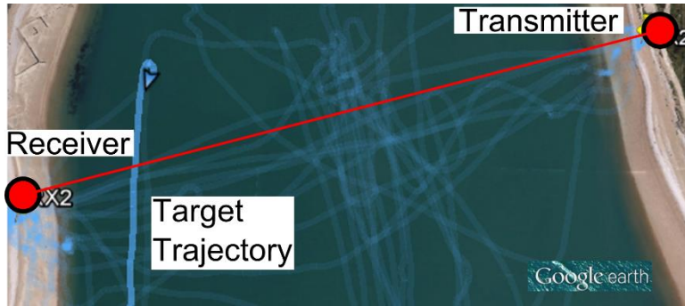
Figure 9 GPS track for second described trial of target crossing nearer to west bank of Langstone Harbour entrance.
