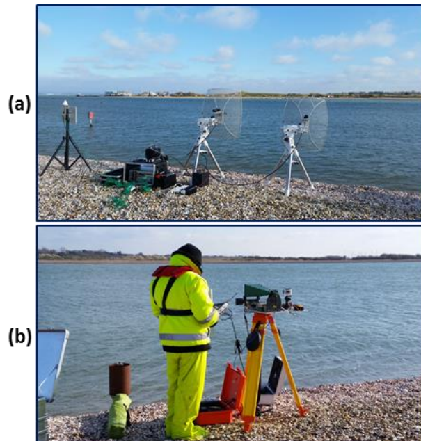
Figure 4 Experimental locations with (a) NetRAD and (b) FSR transmitter node
