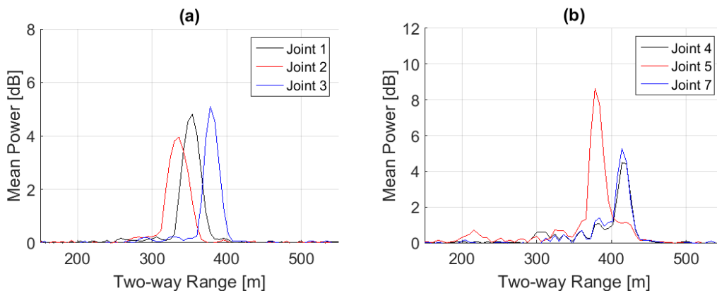
Figure 17 Average range profiles over time period boat target passes in front of Node 3 for (A) No towed sphere target (B) Towed sphere target
