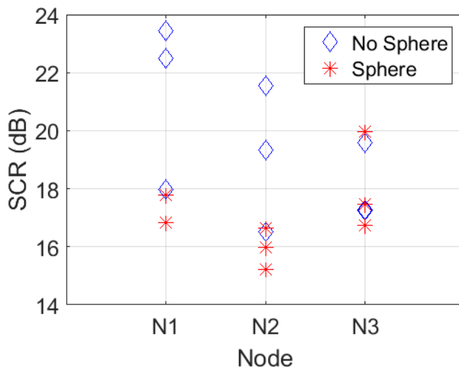
Figure 18. SCR levels for all three NetRAD Radar Nodes when measuring the target with and without the towed sphere As mentioned in Section 3.1, the signals from the FSR system are time domain Doppler signatures, which are formed in the regions close to and as targets cross the baseline. The formation is fundamentally due to
