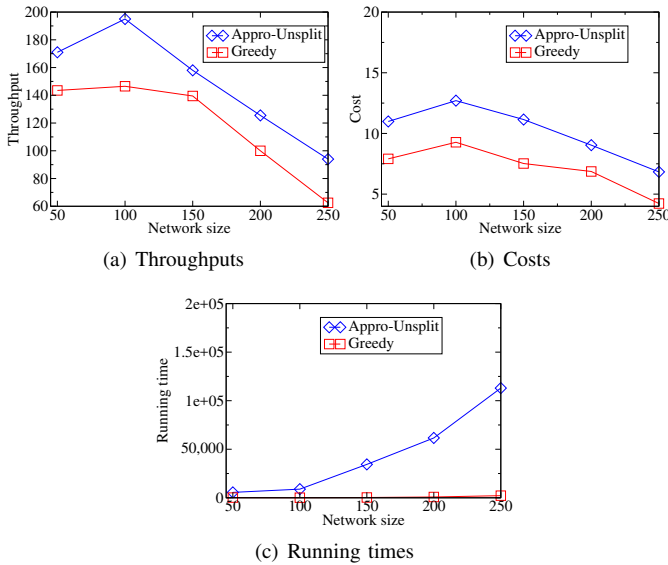
Fig. 5. The performance of algorithms Appro-Unsplit and Greedy.
