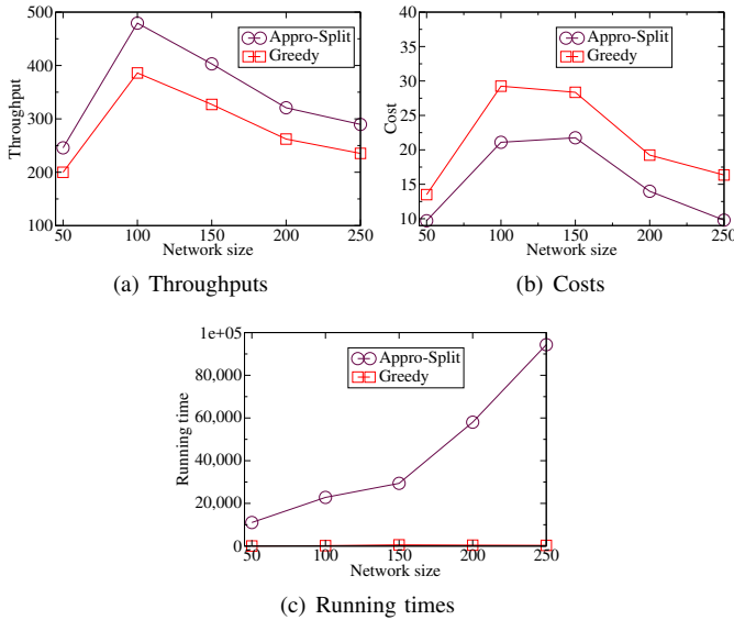
Fig. 4. The performance of algorithms Appro-Split and Greedy. comparing the performance of algorithm Appro-Split and algorithm Appro-Unsplit in Fig. 4 and Fig. 5, it can be seen that algorithm Appro-Split admits more requests than algorithm Appro-Unsplit.
