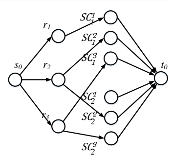
Fig. 2. A constructed auxiliary graph G' based on a network with two data centers DC_1 and DC_2 and three requests to be admitted, i.e., r_1 , r_2 , and r_3 , where requests r_1 , r_2 , and r_3 require instances of type 1, 2, and 3 service chains, respectively, and DC_2 is too far from the source of r_1 to meet its delay requirement.
