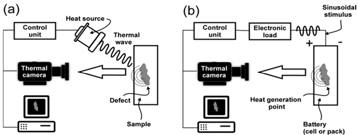
Figure 8. Overview of lock-in thermography process highlighting (a) the traditional use of a heat lamp to detect subsurface defects and (b) the modified use of the direct electrical current employed by Robinson et al. [57].
