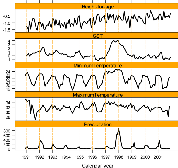
Figure 1 Climate and HAZ in Tumbes. Units for y-axis: height-for-age Z-score (HAZ), sea surface temperature (SST, degrees Celsius), minimum and maximum temperatures (degrees Celsius), and precipitation (mm). Precipitation and temperature data for Tumbes for 1991–2001 were obtained from the Peruvian National Weather Service (SENAMHI). SST data were obtained from the International Institute of Climate and Society (IRI).
