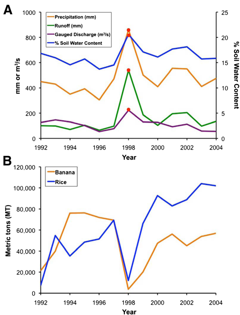
Figure 2 Moisture and subsequent agricultural impact in Tumbes. A. Annual precipitation from NASA's Modern-Era Reanalysis for Research and Applications, runoff (Noah Land Surface Model hydrological simulation), gauged discharge (Tigre gauging station), and percent soil water content (Noah Land Surface Model) for the Tumbes River basin for the 6 years preceding and following the 1997-1998 El Niño event. Values in 1998, indicated in red, are two standard deviations above the mean for all variables. B. Annual banana and rice production in Tumbes (Peruvian Ministry of Agriculture).
