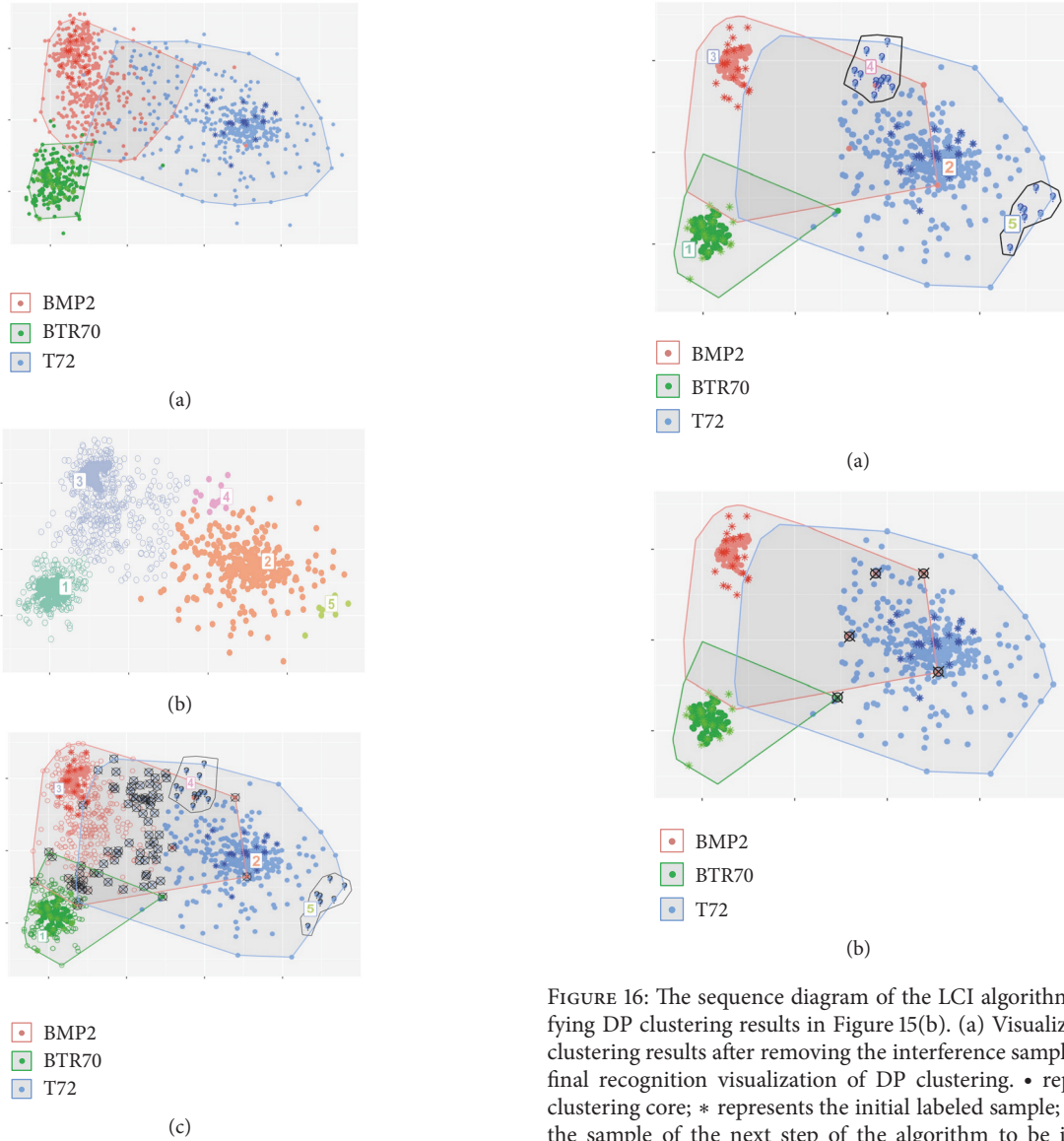
FIGURE 15: In EOC 1 experiment, the visualization results of the first two steps of the S^2DP and WKFDA+DP+S^3VM algorithms when the number of the samples is 21. (a) WKFDA features: • represents the learning set and * represents the initial labeled samples; (b) actual classification map of WKFDA features after DP clustering has been carried: • represents the clustering core and ◦ represents the clustering halo; (c) true classification map of (b): • represents the clustering core, ⊗ represents the clustering error sample, and ? represents the sample of the next step of the algorithm to be identified.
