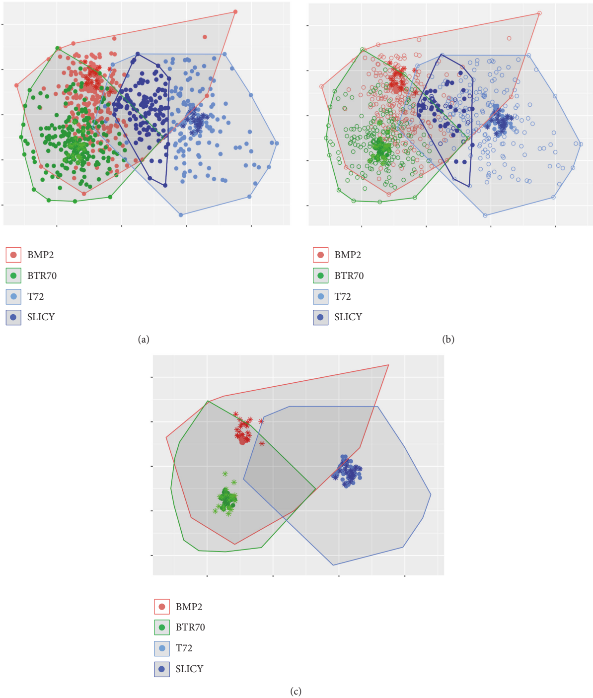
FIGURE 21: Under EOC_2, when the labeled samples number is 21, IS^2DP+S^2DP 's outcomes of the learning set: (a) WKFDA's projection of the learning set; (b) DP clustering result; (c) reliable samples selected and labeled by LCI. Red circle, green circle, light blue, and blue circle represent BMP2, BTR70, T72, and SLICY target samples, respectively, and * represents labeled sample.
