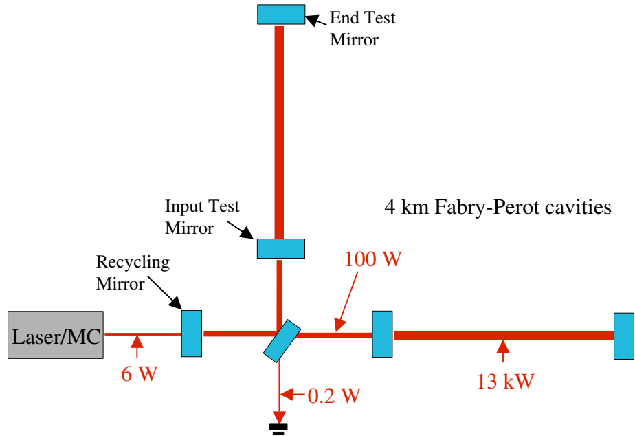
Figure 3. The optical layout of a LIGO interferometer showing the laser power at various points. A Michelson interferometer is supplemented with Fabry-Perot arm cavities 4 km long, and a power recycling mirror to reflect light back into the system as it leaves at the bright port.
