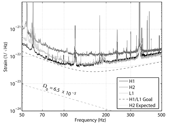
FIG. 1.— Typical strain amplitude spectra of LIGO interferometers during the science run S4 (solid curves top to bottom at 70 Hz: H2, L1, H1). The black dashed curve is the LIGO sensitivity goal for the 4 km interferometers H1 and L1. The black dotted curve is the expected design LIGO sensitivity of the 2 km interferometer H2. The gray dashed curve is the strain amplitude spectrum corresponding to the limit presented in this paper for the frequency-independent GW spectrum \Omega_0 < 6.5 \times 10^{-5} .
