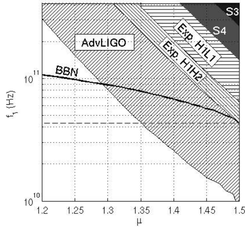
FIG. 16.—The f_1 - \mu plane for the pre-big bang models with f_s = 30 Hz. The shaded regions are excluded by the LIGO S3 limit ( dark gray ) and by the LIGO S4 limit presented here ( light gray ). The hatched regions will be accessible to future LIGO runs: expected LIGO sensitivity for the H1-L1 pair, assuming design interferometer strain sensitivity and 1 yr of exposure ( horizontal hatching ); expected LIGO sensitivity for the H1-H2 pair, assuming design interferometer strain sensitivity and 1 year of exposure ( \\ hatching ); expected Advanced LIGO sensitivity for the H1-H2 pair, assuming interferometer strain sensitivity tuned for the binary neutron star inspiral search and 1 yr of exposure ( /// hatching ). The solid black curve is the exclusion curve based on the BBN limit (the excluded region is above the curve). The horizontal dashed line denotes the most natural value of f_1 = 4.3 \times 10^{10} Hz.
