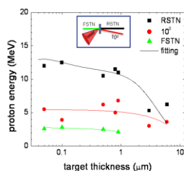
Fig.1 Maximum proton energy variation with target thickness along the measured directions: rear surface target normal (RSTN), 10° to RSTN and front surface target normal (FSTN). The solid line is fit calculated from the model. Other two dashed lines are guide for the eye. Aluminums targets were irradiated under 35° laser incidence
