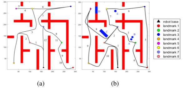
Figure 5. DA-TPP dynamic replanning. (a) initial plan, (b) actual paths executed (unknown obstacles shown in blue)
