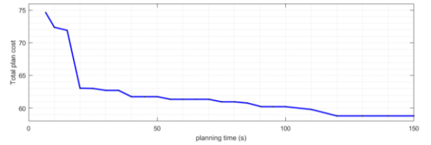
Figure 4. Anytime planning cost reductions
