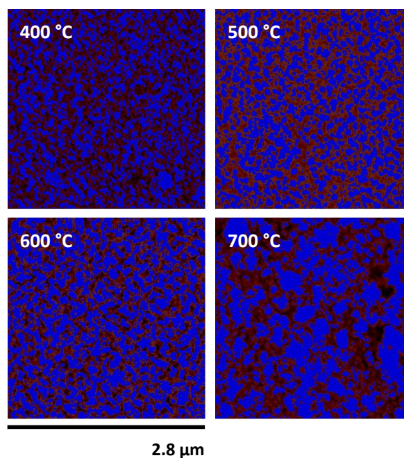
Figure 9. Fibre topography of heat-treated fibres masked to identify the coverage of the structure (sample areas approx. 2.8 \times 2.8 \mu\text{m} ).
