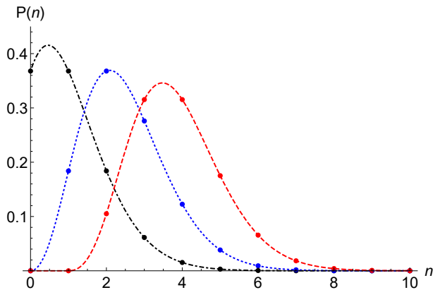
FIG. 3: (color online) The photon number probability distributions for (a) an initial coherent state with a mean photon number of unity (black circles, dash-dotted line) (b) the state produced by a single photon addition (blue circles, dotted line) and (c) the state produced by two photon addition (red circles, dashed line). Photon subtraction leaves the initial coherent-state statistics unchanged.
