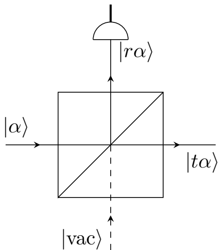
FIG. 2: The action of our photon subtraction process on an initial coherent state |\alpha\rangle .
