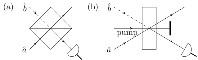
FIG. 1: Schematic for implementations of (a) photon subtraction using a weakly reflecting beam splitter and (b) photon addition using a weak parametric amplifier.
