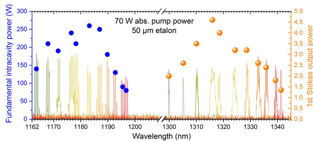
Fig. 6. Wavelength tuning of the fundamental laser (blue circles) with related tuning of the first-Stokes Raman laser (orange) at 70 W of absorbed diode pump power and corresponding log-scaled output spectra.
