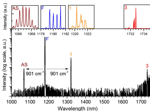
Fig. 4. Emission spectrum (0.2 nm resolution) of the SDL-pumped Raman laser for 92 W of absorbed diode pump power and an all-HR cavity. AS, anti-Stokes; F, fundamental; “1” and “3,” first- and third-Stokes lasers. Top insets: 0.05 nm resolution.
