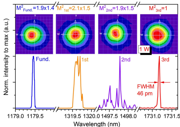
Fig. 9. Spectra of the cascaded Raman lasers collected by an optical spectrum analyzer with 50 pm resolution limit, with 1 W third-Stokes output power. Insets: spatial profiles of the filtered output beams at the fundamental and Raman wavelengths.
