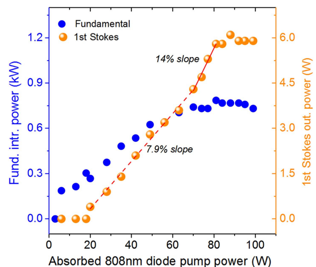
Fig. 5. Power transfer characteristic of the Raman laser and the fundamental intracavity power.
