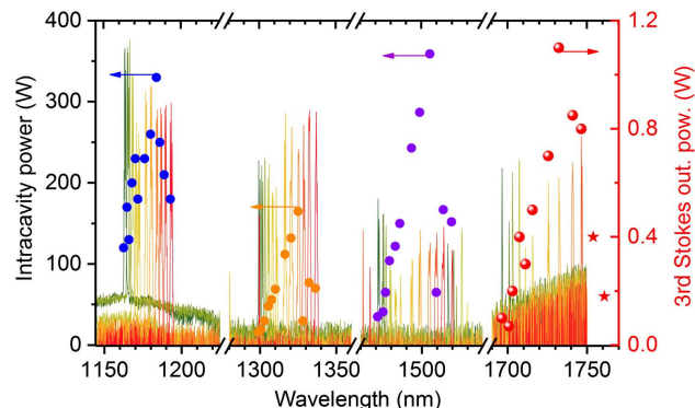
Fig. 10. Tuning of the fundamental and the cascaded Raman laser for an absorbed diode pump power of 84 W and corresponding log-intensity emission spectra (varying from green to red for increasing fundamental wavelength) measured with 0.2 nm resolution. Red stars: calculated wavelength as out of range of the optical spectrum analyzer.
