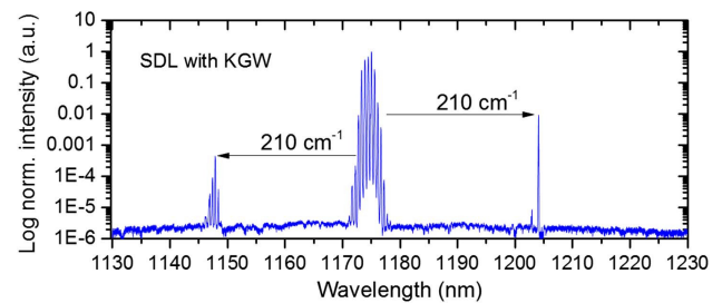
Fig. 3. Section of an emission spectrum of the intracavity-pumped KGW Raman laser obtained at high pump power.
