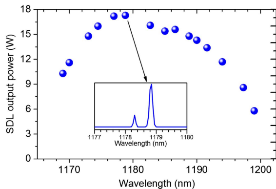
Fig. 1. Tuning curve of the SDL for 95 W absorbed pump power and 1.6% output coupling, obtained via rotation of an intracavity birefringent filter. Inset: SDL emission spectrum at the highest output power.
