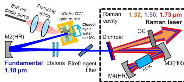
Fig. 2. Schematic of the SDL-pumped KGW Raman laser. HR, high reflector; OC, output coupler; DBR, distributed Bragg reflector; HS, heat spreader.
