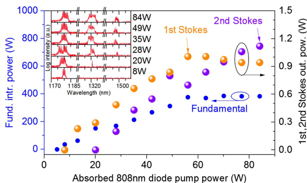
Fig. 7. Output power of the cascaded Raman at the first- and second-Stokes radiation (orange and purple spheres, respectively), and dependency of the fundamental intracavity power on the absorbed diode pump power (blue circles). Inset: Fundamental, first- and second-Stokes Raman spectra at different absorbed pump powers.
