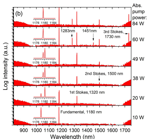
Fig. 8. (a) Power transfer of the third-Stokes Raman laser (red spheres); and intracavity power of the fundamental (blue squares), first-Stokes (orange circles), and second-Stokes (purple triangles). (b) Evolution of the emission spectra of the Raman laser taken with 0.2 nm resolution.
