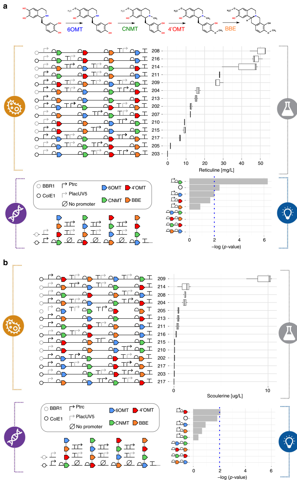
Fig. 4 Combinatorial optimization of the ( S )-reticuline/( S )-scoulerine pathway through the Design/Build/Test/Learn cycle. a A biosynthetic pathway composed of four enzymes from Coptis japonica (6OMT, CNMT, 4'OMT, and BBE; see Supplementary Table 10) was selected. For this DBTL cycle, a combinatorial library totaling 2592 pathway configurations was designed by varying the order of pathway genes, promoter parts ( P_{trc} and P_{lacUV5} ) and plasmid copy numbers (pBBR1 and ColE1 origins). Through the application of statistical DoE, the designed library was reduced to 16 representative constructs, of which 14 were successfully assembled and tested. This pathway library was expressed in E. coli DH5 \alpha and reticuline titers were quantified. Statistical analysis was then used to assess the relative effects of the different design factors tested. b Quantification of scoulerine titers observed for the same 14 constructs and statistical analysis of the relative effects of the different design factors
