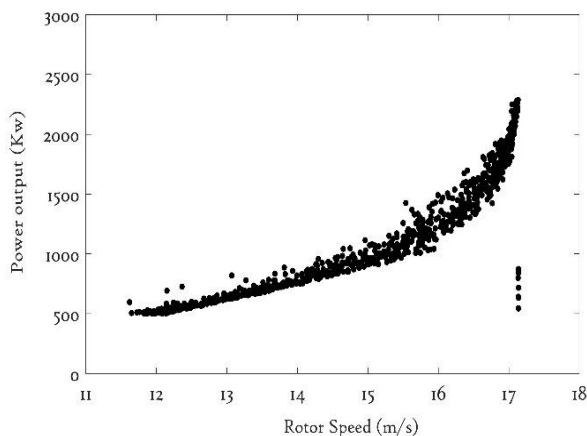
Figure 3: Filtered rotor power curve
