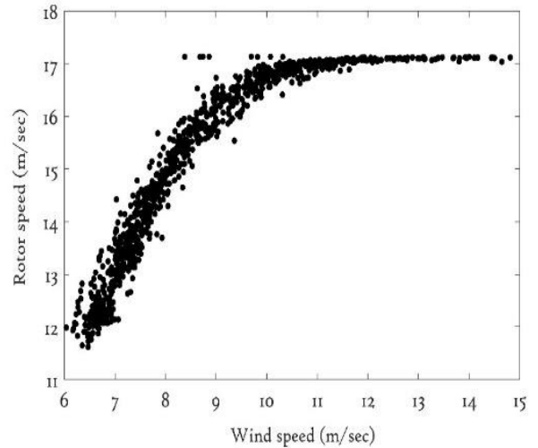
Figure 4: Filtered rotor speed curve
