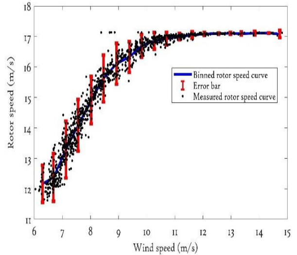
Figure 8: Binned Rotor speed curve
