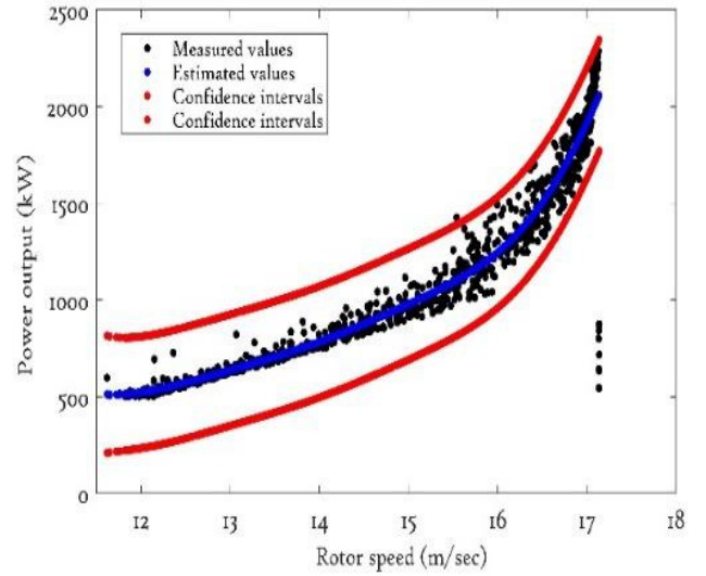
Figure 5: GP rotor power curve
