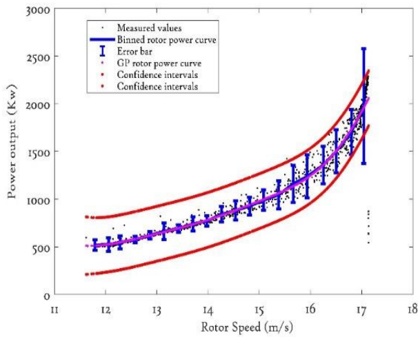
Figure 9: Comparative analysis of rotor power curve based on GP and binning
