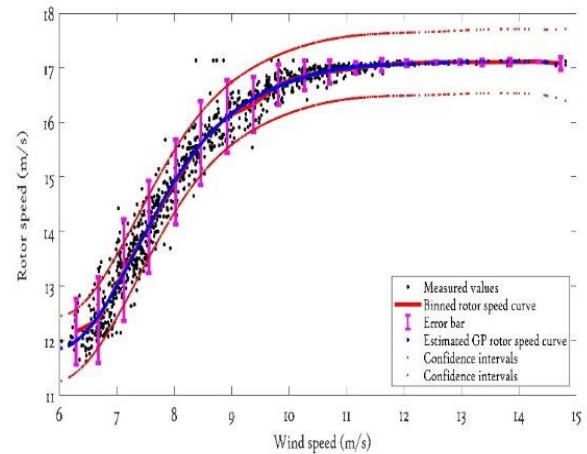
Figure 10: Comparative analysis of rotor speed curve based on GP and binning
