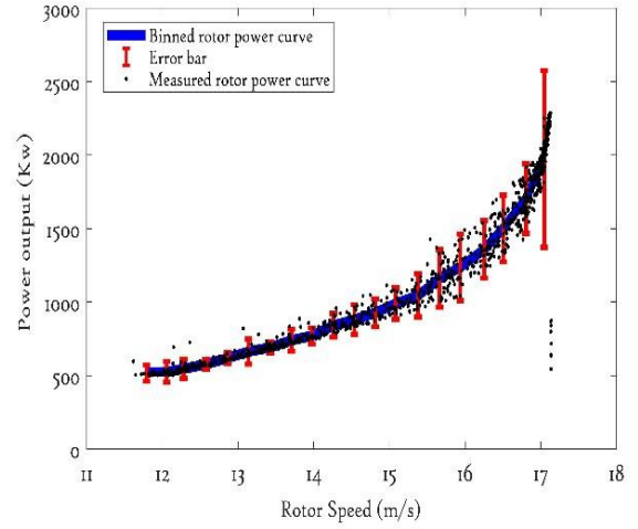
Figure 7: Binned rotor power curve
