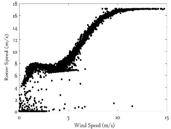
Figure 2: Rotor speed curve
