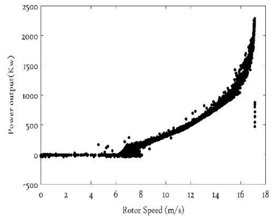
Figure 1: Rotor power curve
