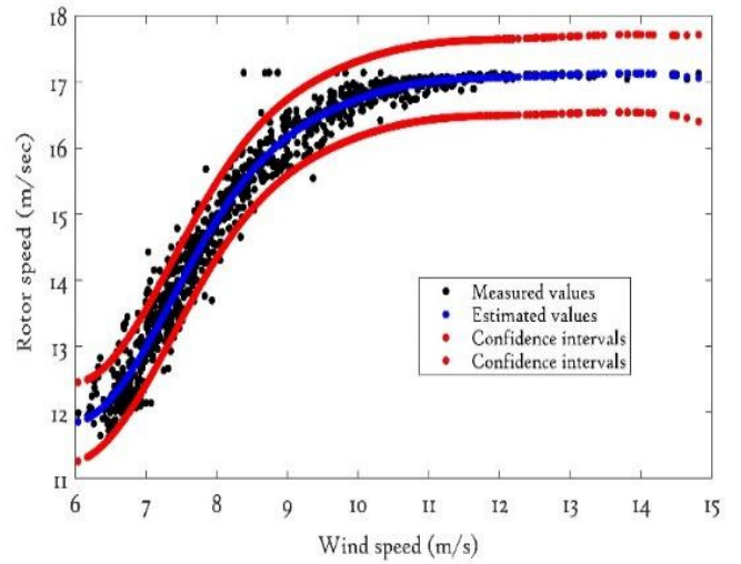
Figure 6: GP Rotor speed curve
