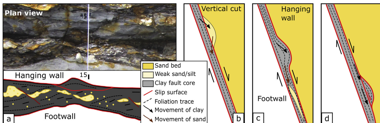
Fig. 13. Field example and cartoon of the sidewall ripout mechanism. a) Picture (top) and map (bottom) of an along-strike section of section 1; Cartoon: a weaker area on the hanging wall (b) is eroded away and incorporated as a sand lens (c) as the space is filled by foliated clay. d) The infill-area is subsequently cut-off from the main fault core by a straighter slip surface or shear zone.
