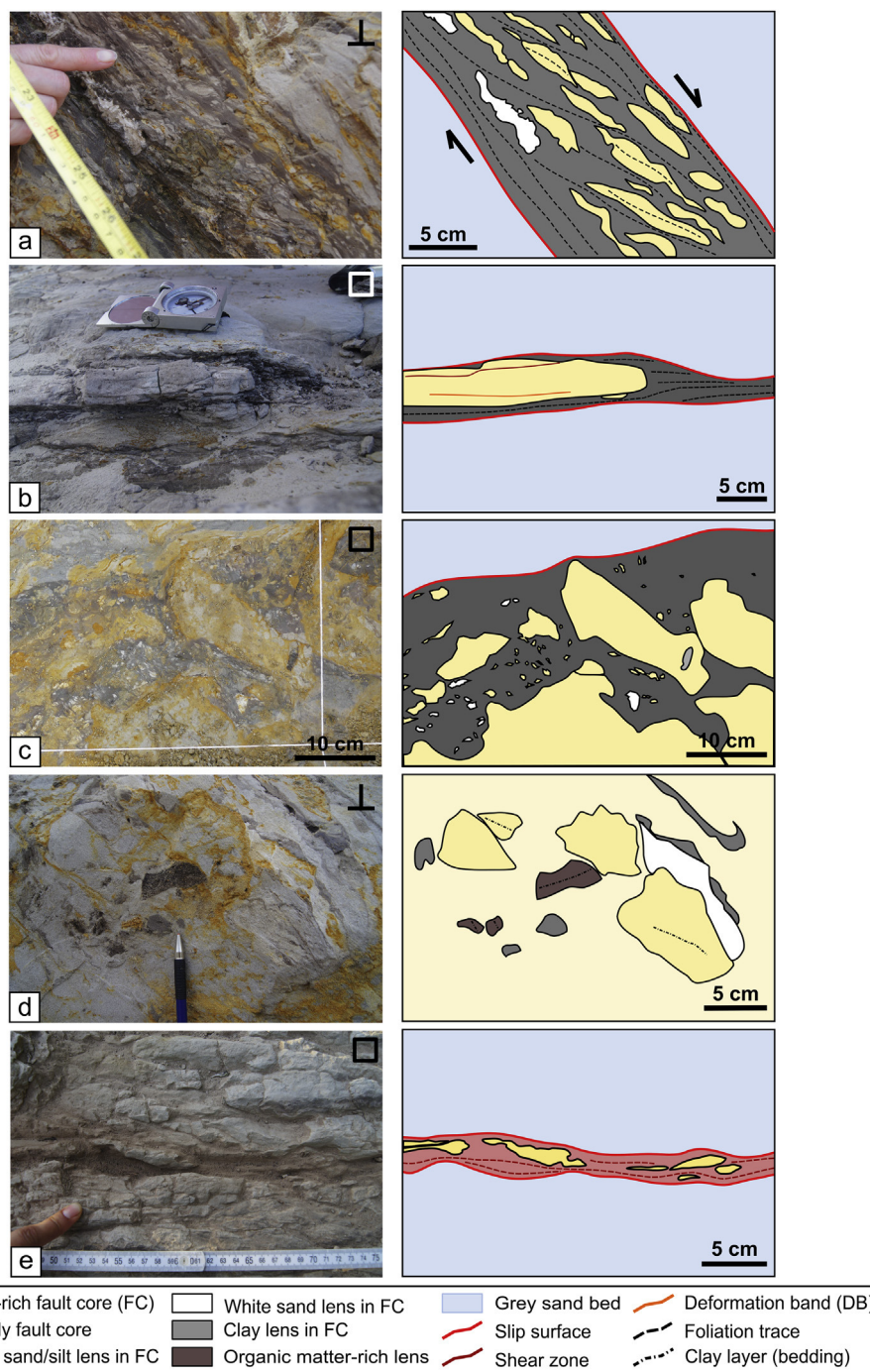
Fig. 9. Fault core types identified along the main fault, picture on the left and sketch on the right. a) Foliated clay-rich fault core and elongate sand lenses (section 2). b) Thin, foliated clay-rich fault core with sand lens in the middle (section 1). c) Chaotic clay-rich fault core with irregular sand lenses (section 3). d) Sandy breccia fault core with clasts of different composition and orientation (section 4). e) Anastomosing sandy and silty shear zone fault core, with weakly deformed sand lenses (section 1). Outcrop orientation: □ indicates plan view; ⊥ indicates sub-vertical view.
