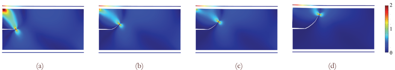
Figure 13: Point opening force: Von Mises contour plots and crack evolution for different loading steps.
