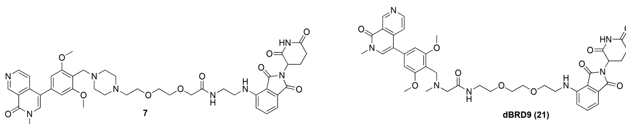
Figure 3. Structures of compounds 7 and 21. 18
