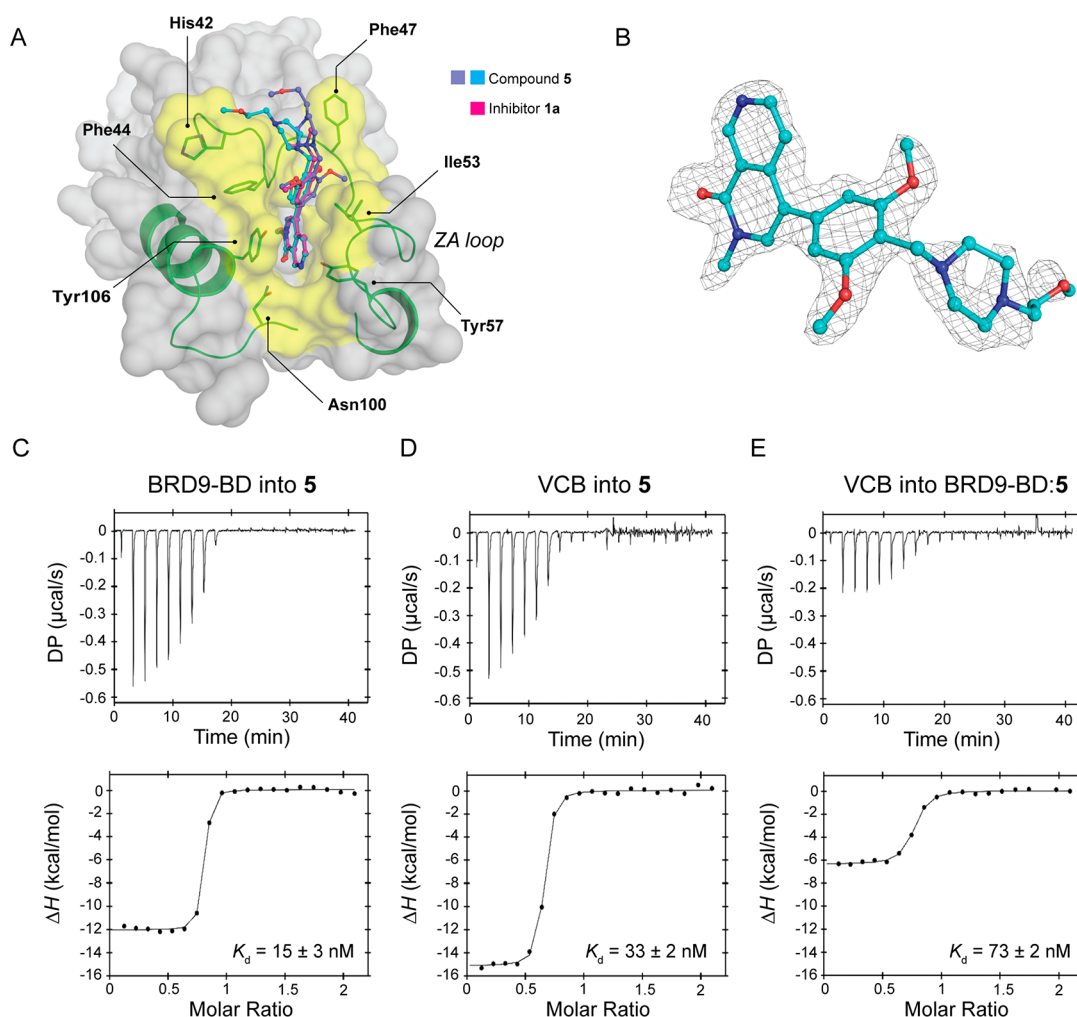
Figure 4. Ternary complex formation and analysis of binding mode for compound 5 . (A) Cocrystal structure of BRD9-BD and compound 5 . The warhead component of the degrader (purple and cyan; one from each protomer in the ASU) recapitulates the binding of inhibitor 1a (magenta, PDB code 5EUI), 56 whereas the alkylated piperazine used to attach the linker is solvent-exposed and does not form any unfavorable interactions with the protein. (B) F_o - F_c omit map of compound 5 (contoured at 2.5\sigma ) showing electron density for the alkylated piperazine ring. (C) BRD9-BD titrated into 5 alone. (D) VCB titrated into 5 alone. (E) VCB titrated into BRD9-BD: 5 binary complex. VCB binds more weakly to the binary complex BRD9-BD: 5 ( K_d = 73 nM) compared to compound 5 alone ( K_d = 33 nM), indicating negative cooperativity.
