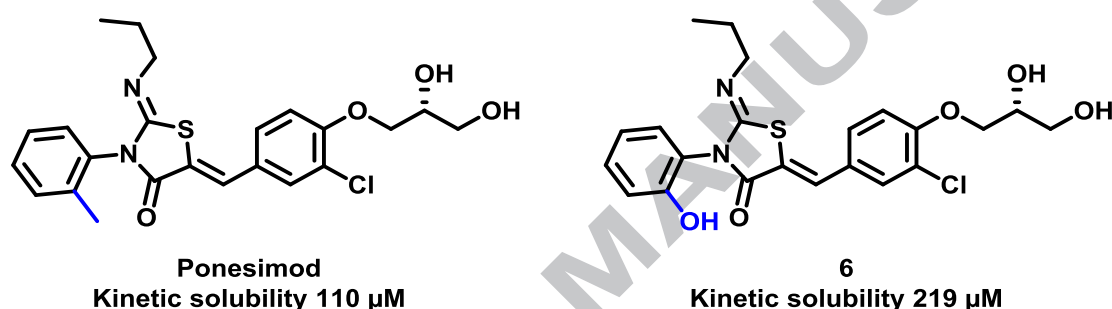
Figure 2. Improvements in aqueous kinetic solubility from introduction of o -phenol group
