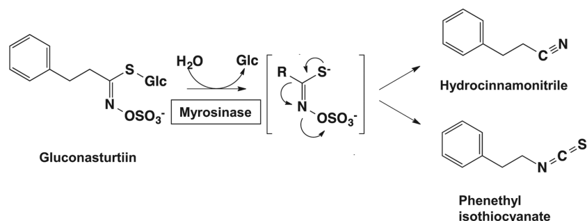
Figure 1. The myrosinase reaction. The glucosinolate gluconasturtiin is hydrolytically cleaved by the enzyme myrosinase to give an unstable aglycone and liberate glucose. The reaction product spontaneously rearranges into hydrocinnamitrile and phenethyl isothiocyanate (PEITC).
