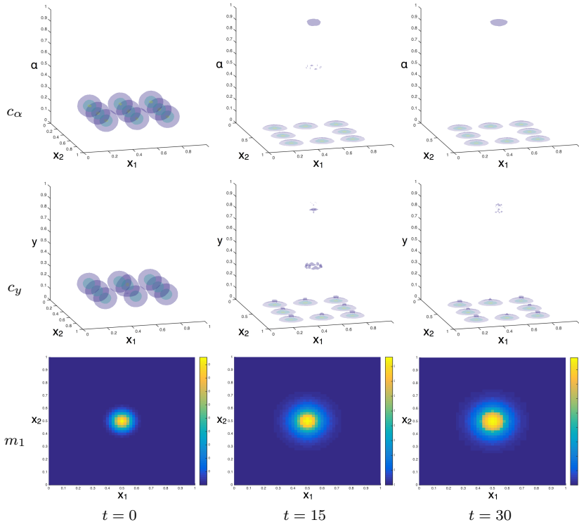
Fig. 7: Multi-cluster results from simulation of model (28) for high affinity ( \lambda = 0.5 ) are given for c(t, x, y, \alpha) in the spatio-metabolic domain (1 st row, c_\alpha ), with x on the horizontal plane and \alpha on the vertical axis; in the spatio-binding domain (2 nd row, c_y ), with x on the horizontal plane and y on the vertical axis; and for m(t, x) in space (3 rd row), for t \in \{0, 15, 30\} respectively.
