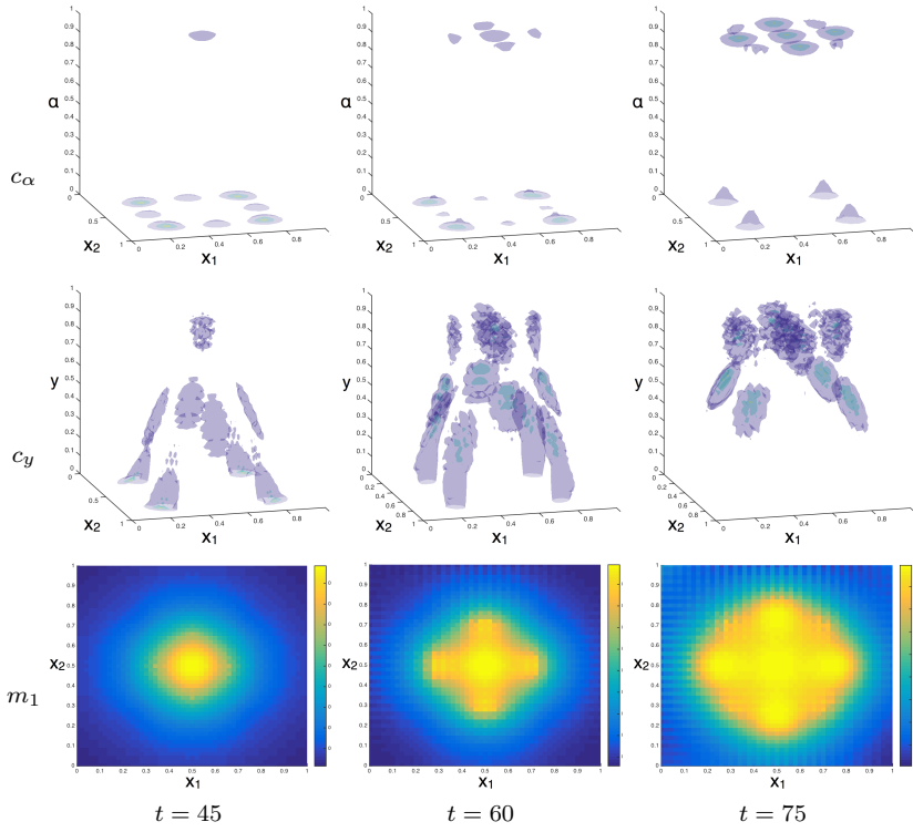
Fig. 6: Multi-cluster results from simulation of model (28) for low affinity ( \lambda = 0.01 ) are given for c(t, x, y, \alpha) in the spatio-metabolic domain (1 st row, c_\alpha ), with x on the horizontal plane and \alpha on the vertical axis; in the spatio-binding domain (2 nd row, c_y ), with x on the horizontal plane and y on the vertical axis; and for m(t, x) in space (3 rd row), for t \in \{45, 60, 75\} respectively.
