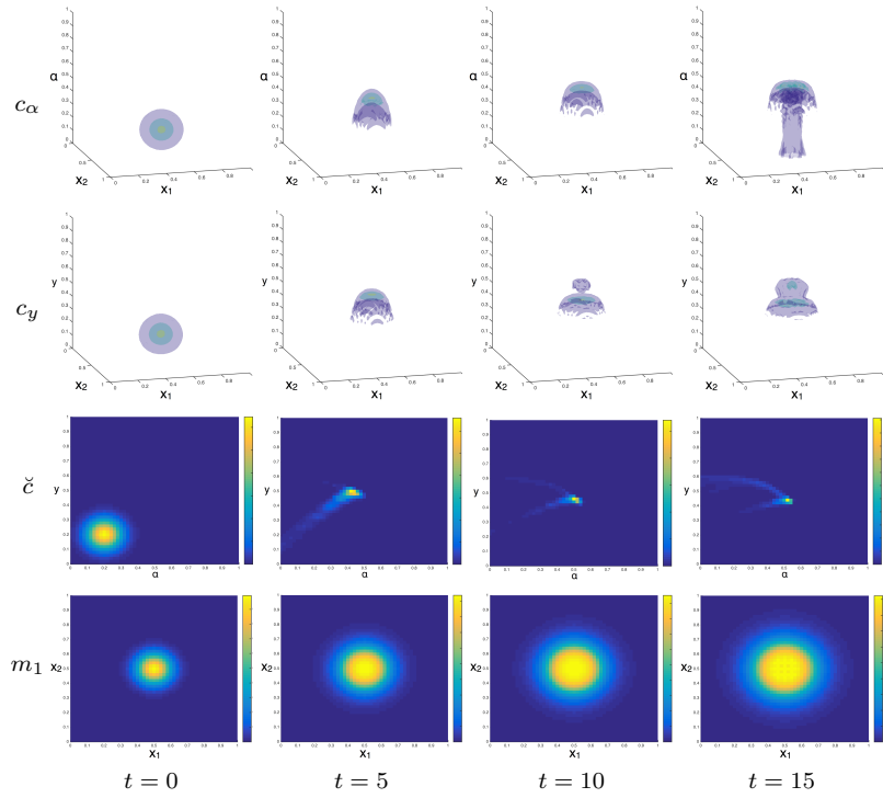
Fig. 3: Single-cluster results from simulation of model (27) for low affinity ( \lambda = 0.1 ) are given for c(t, x, y, \alpha) in the spatio-metabolic domain (1 st row, c_\alpha ), with x on the horizontal plane and \alpha on the vertical axis; in the spatio-binding domain (2 nd row, c_y ), with x on the horizontal plane and y on the vertical axis; in the metabolo-binding domain (3 rd row, \check{c} ), with \alpha on the horizontal axis and y on the vertical axis; and for m(t, x) in space (4 th row), for t \in \{0, 5, 10, 15\} respectively.
