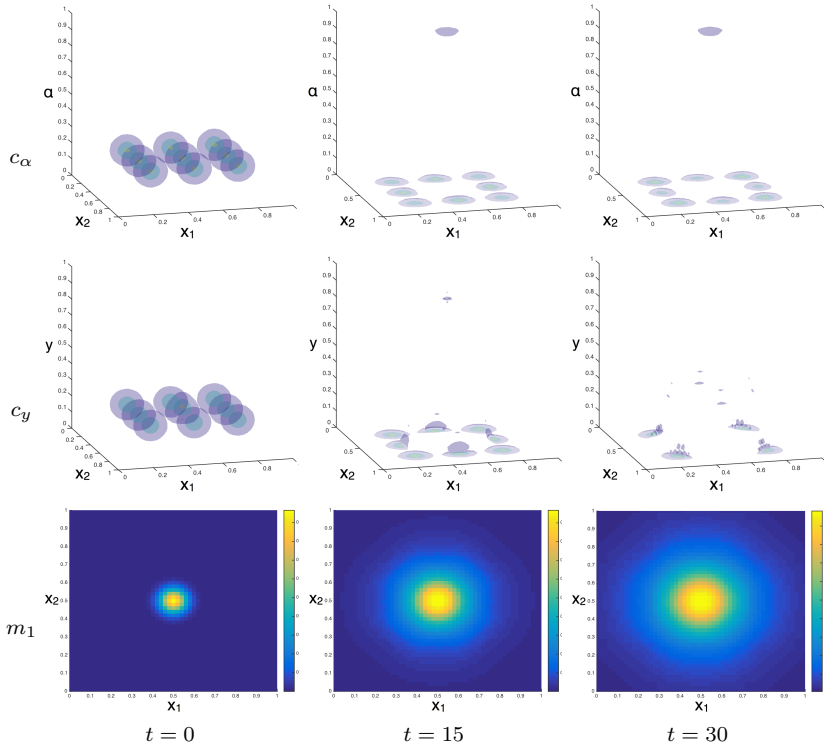
Fig. 5: Multi-cluster results from simulation of model (28) for low affinity ( \lambda = 0.01 ) are given for c(t, x, y, \alpha) in the spatio-metabolic domain (1 st row, c_\alpha ), with x on the horizontal plane and \alpha on the vertical axis; in the spatio-binding domain (2 nd row, c_y ), with x on the horizontal plane and y on the vertical axis; and for m(t, x) in space (3 rd row), for t \in \{0, 15, 30\} respectively.
