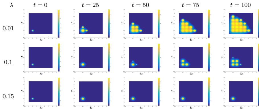
Fig. 1: Multi-cluster results in the concentration of molecular species m(t, x) from simulation of the simple model (1) for varying affinities, \lambda \in \{0.01, 0.1, 0.15\} , and for t \in \{0, 25, 50, 75, 100\} respectively.
