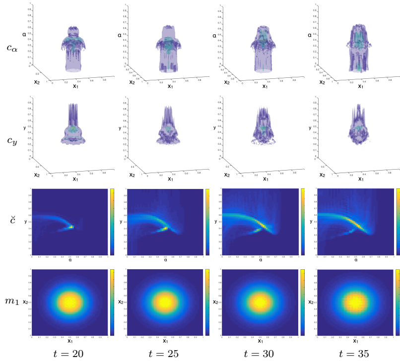
Fig. 4: Single-cluster results from simulation of model (27) for low affinity ( \lambda = 0.1 ) are given for c(t, x, y, \alpha) in the spatio-metabolic domain (1 st row, c_\alpha ), with x on the horizontal plane and \alpha on the vertical axis; in the spatio-binding domain (2 nd row, c_y ), with x on the horizontal plane and y on the vertical axis; in the metabolo-binding domain (3 rd row, \check{c} ), with \alpha on the horizontal axis and y on the vertical axis; and for m(t, x) in space (4 th row), for t \in \{20, 25, 30, 35\} respectively.
