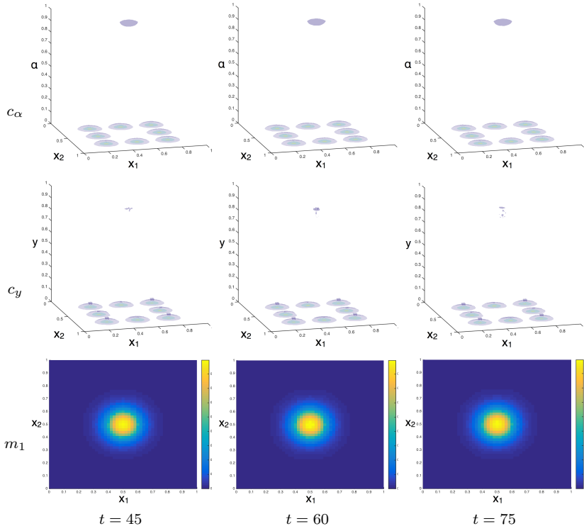
Fig. 8: Multi-cluster results from simulation of model (28) for high affinity ( \lambda = 0.5 ) are given for c(t, x, y, \alpha) in the spatio-metabolic domain (1 st row, c_\alpha ), with x on the horizontal plane and \alpha on the vertical axis; in the spatio-binding domain (2 nd row, c_y ), with x on the horizontal plane and y on the vertical axis; and for m(t, x) in space (3 rd row), for t \in \{45, 60, 75\} respectively.
