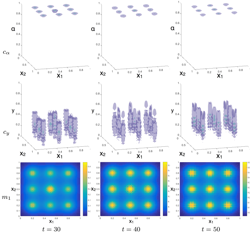
Fig. 10: Multi-cluster results from simulation of model (29) for high affinity ( \lambda = 0.5 ) are given for c(t, x, y, \alpha) in the spatio-metabolic domain ( 1^{st} row, c_\alpha ), with x on the horizontal plane and \alpha on the vertical axis; in the spatio-binding domain ( 2^{nd} row, c_y ), with x on the horizontal plane and y on the vertical axis; and for m(t, x) in space ( 3^{rd} row), for t \in \{30, 40, 50\} respectively.
