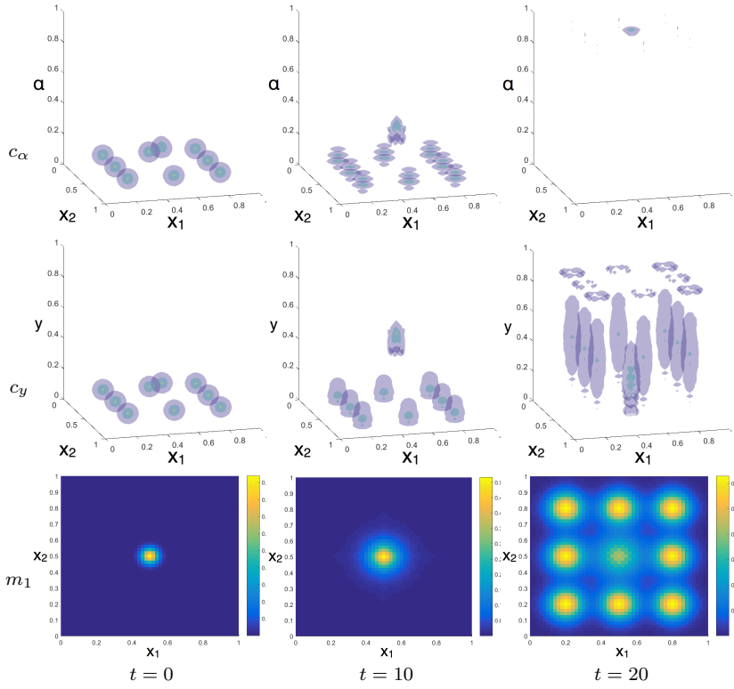
Fig. 9: Multi-cluster results from simulation of model (29) for high affinity ( \lambda = 0.5 ) are given for c(t, x, y, \alpha) in the spatio-metabolic domain ( 1^{st} row, c_\alpha ), with x on the horizontal plane and \alpha on the vertical axis; in the spatio-binding domain ( 2^{nd} row, c_y ), with x on the horizontal plane and y on the vertical axis; and for m(t, x) in space ( 3^{rd} row), for t \in \{0, 10, 20\} respectively.
