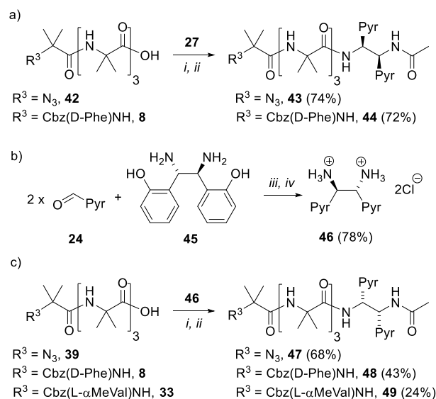
Scheme 6. Synthesis of uncontrolled foldamers 43 and 47 , D-Phe controlled foldamers 44 and 48 , and L- \alpha -MeVal controlled foldamer 49 . a,c) i , EDC/HOBt, i -Pr 2 NEt, CH 2 Cl 2 ; ii , Ac 2 O, CH 2 Cl 2 . b) iii , DMSO, 3 h, then H 2 O. iv THF, conc. HCl.
