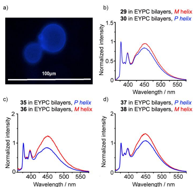
Fig. 8. a) Epi-fluorescence microscopy image of EYPC GUVs with 37 embedded in the bilayers at 1 mol%; (b-d) Normalized fluorescence emission spectra for 29 , 30 , 35 - 38 (10 \mu M, in EYPC LUVs, 800 nm diameter at 1 mol %, emission normalized to 377 nm).
