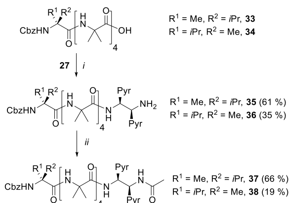
Scheme 4. Synthesis of α-MeVal controlled foldamers 35 – 38 . i , EDC/HOBt, i -Pr 2 NEt, CH 2 Cl 2 ; ii , Ac 2 O, CH 2 Cl 2 .
