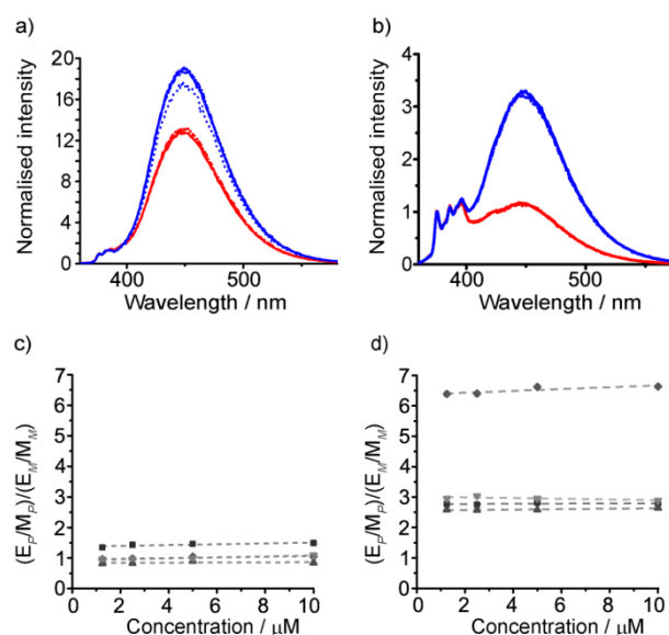
Fig. 4. a,b) Fluorescence emission spectra (normalized to 1 at 377 nm) in MeOH of a) amino-terminated foldamers 35 ( P helix, blue trace) and 36 ( M helix, red trace); b) acetamide-terminated foldamers 37 (blue) and 38 (red) in MeOH. Spectra shown for 10 μM (solid line) 5 μM (dashed line) 2.5 μM (dash-dotted line) and 1.25 μM (dotted line) of compound; c,d) Sensitivity ratio ( S_R ) values for c) 35 and 36 ; d) 37 and 38 . S_R = ([E/M \text{ for } P]/[E/M \text{ for } M]) for the diastereomeric pairs in CH 2 Cl 2 (◆) MeOH (■) MeCN (▲) and THF (▼) at different concentrations. For 35 and 36 the response in CH 2 Cl 2 is identical to that in THF.
