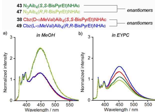
Fig. 9. Normalized fluorescence emission spectra (emission normalized to 1 at 377 nm) for 43 (dark green line), 47 (pale green line), 38 (red line) and 49 (blue line) in a) MeOH (10 \mu M); b) EYPC LUVs, 800 nm diameter at 1 mol % (10 \mu M).
