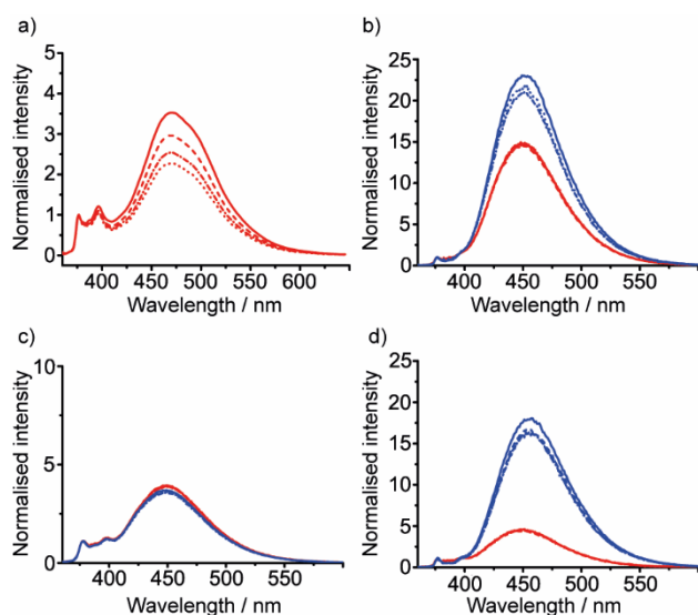
Fig. 3. Emission spectra normalized to 1 at 377 nm from a) 31 in MeOH; b) 29 ( M helix, red traces) and 30 ( P helix, blue traces) in MeOH; c) 29 (red traces) and 30 (blue traces) in CH 2 Cl 2 ; d) 29 (red traces) and 30 (blue traces) in MeCN. Foldamer concentrations: 10 μM (solid line) 5 μM (dashed line) 2.5 μM (dash-dotted line) and 1.25 μM (dotted line).
