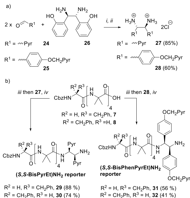
Scheme 3. a) Synthesis of ‘third generation’ probes 27 and 28 . Pyr = pyren-1-yl. i , DMSO, 3 h. then H 2 O. ii THF, Conc. HCl; b) Synthesis of foldamers 29–32 bearing third generation probes. iii , HOBt, EDC.HCl, CH 2 Cl 2 . iv , i -Pr 2 NEt, RT, 2 d.
