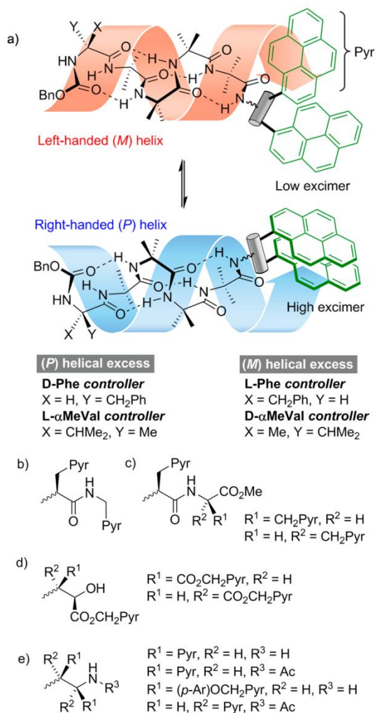
Fig. 1. Development of chiral, conformationally responsive fluorescent probes. Pyr = pyren-1-yl. p -Ar = 1,4-disubstituted benzene. (a) Schematic bis(pyrenyl-yl) probe attached to M and P screw-sense conformers of a controlled Aib 4 helix; (b),(c) Reporters incorporating one or two pyrenylalanine (Pya) residues; (d) Reporters derived from aminoalcohol probes; (e) Reporters derived from 1,2-bis(aryl)ethylenediamine probes.
