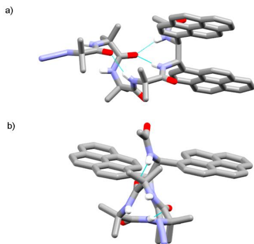
Fig. 5. X-ray crystal structure of 43 a) Viewed side-on, showing M helical structure with bifurcated NH bond between the carbonyl of Aib-2 and the amide NHs of the probe; b) Viewed along the helix axis from N- to C-terminus, revealing the large separation of the pyrene groups.
