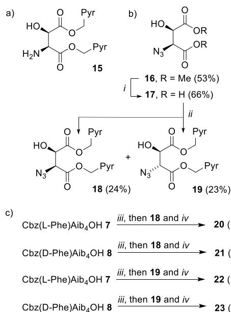
Scheme 2. a) Example of a bis(pyrene) aminoalcohol probe for attachment to the C-terminus of foldamers; b) Synthesis of ‘second generation’ probes 18–19 . Pyr = pyren-1-yl. i , LiI, THF reflux, 48 h then 1 M HCl. ii , 1-(Bromomethyl)pyrene, Et 3 N, MeCN, reflux, 72 h; c) Coupling to foldamers 7 and 8 , iii , EDC, HOBt, THF, RT, 30 min. iv , Et 3 N, THF, RT, 16 h.
