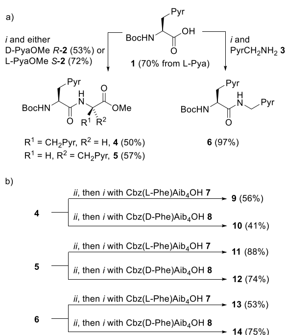
Scheme 1. a) Synthesis of 'first generation' probes 4–6. Pyr = pyren-1-yl. i , EDC, HOBT, i -Pr 2 NEt, CH 2 Cl 2 , RT. b) Synthesis of foldamers 9–14 bearing first generation probes. ii , TFA/CH 2 Cl 2 .
