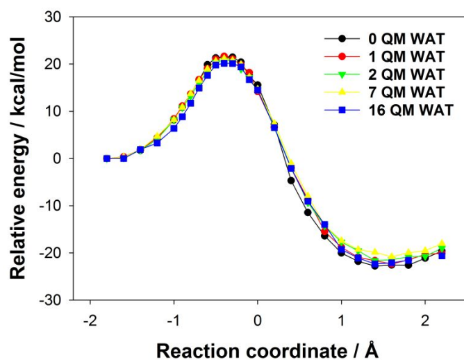
30 31 32 33 34 35 36 37 38 39 40 41 42 43 44 45 46 47 Figure 6. Potential energy profiles for the rearrangement of chorismate to prephenate in 48 solution calculated using projector-based embedding of the SCS-MP2 method in B3LYP with 49 different numbers of DFT water molecules in sub-system B, using the cc-pVDZ basis set. The 50 geometries are taken from B3LYP/6-31G(d)/CHARMM27 pathway calculations treating 51 chorismate and the stated number of water molecules by QM. All energies are relative to the 52 reactant ( r = -1.8 \text{ \AA} ). 53 54 55 56 57 58 59 60
