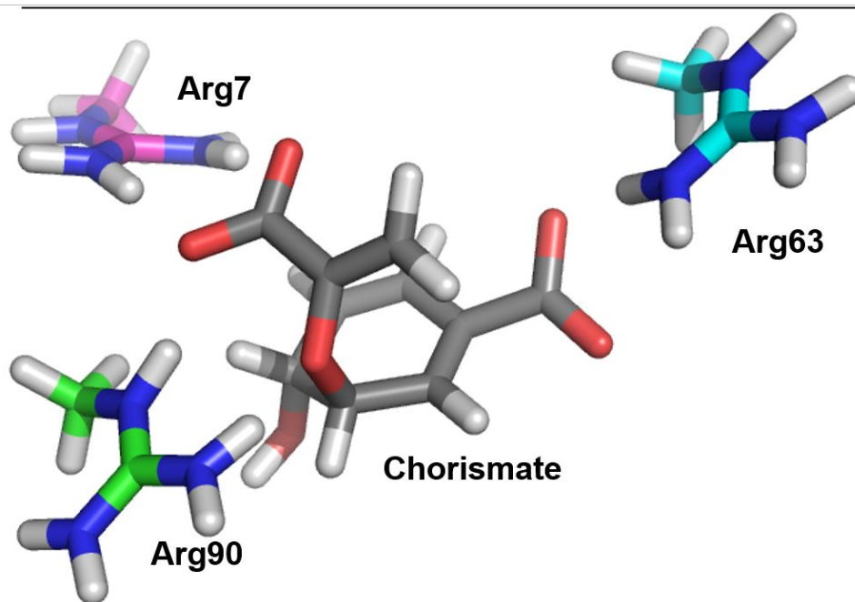
Figure 3. The different QM regions used in projector-based embedding calculations of the reaction in the BsCM enzyme. In all calculations, sub-system A contains only chorismate (grey carbons). One, two or three arginine residues are included in sub-system B and treated by DFT.
