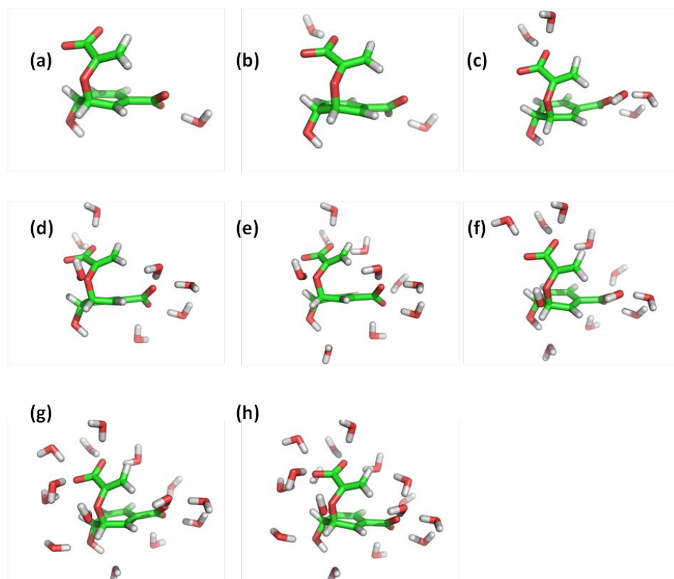
39 40 Figure 2. The different QM regions used in B3LYP QM/MM calculations of the conversion 41 of chorismate to prephenate in water (MM atoms not shown). Increasing numbers of water 42 molecules were treated by QM (in addition to chorismate) in each case: (a) water molecules 43 within distance 1.64 Å (1 water molecule), (b) within 1.67 Å (2 water molecules), (c) 44 within 1.71 Å (5 water molecules), (d) within 1.73 Å (7 water molecules), (e) within 1.74 Å (10 water 45 molecules), (f) within 1.75 Å (11 water molecules), (g) within 1.77 Å (14 water molecules) and 46 (h) within 1.80 Å (16 water molecules). 47 48
