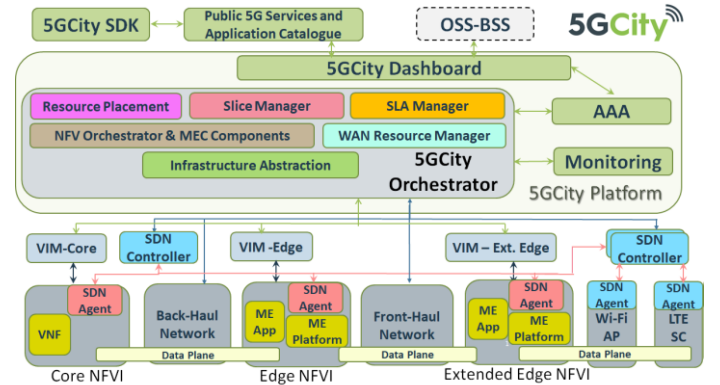
Figure 3. H2020 5GCity architecture [44].
