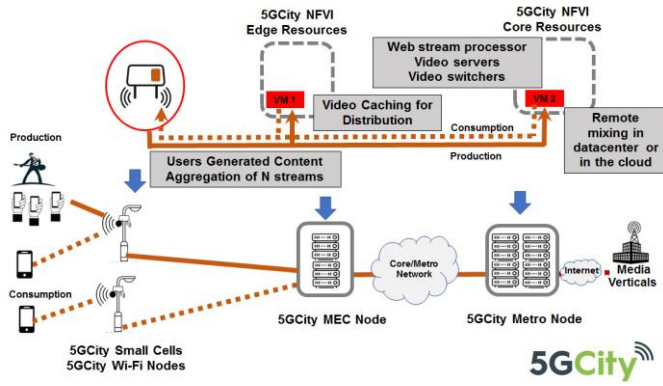
Figure 7. Deploying the UC#1 service chain with 5GCity in Bristol.
