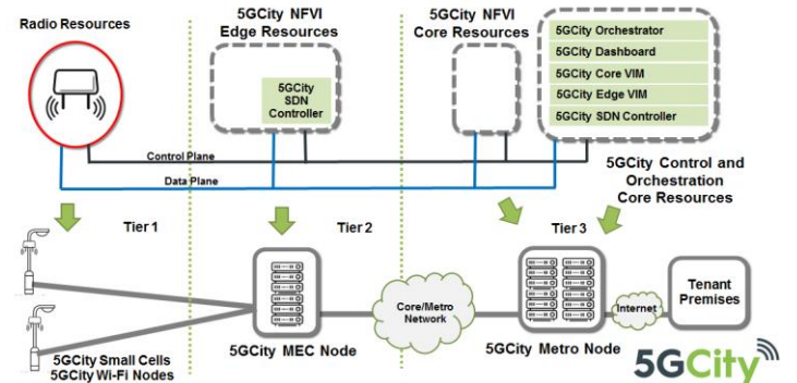
Figure 4. Mapping of 5GCity architecture into a the three-tier candidate city infrastructure [46].
