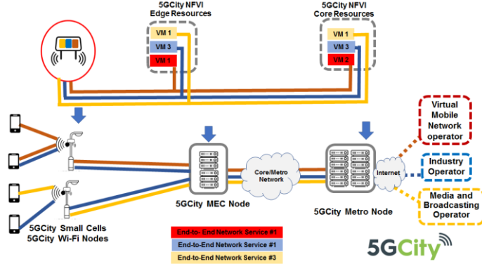
Figure 5. Enablement of end-to-end network services by the 5GCity platform.
