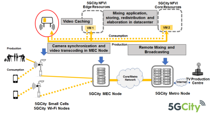
Figure 11. Deploying the UC#3 service chain with 5GCity in Barcelona.
