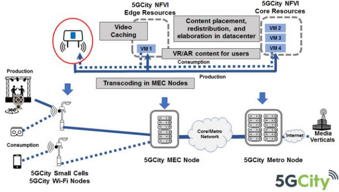
Figure 9. Deploying the UC#2 service chain with 5GCity in Lucca.
