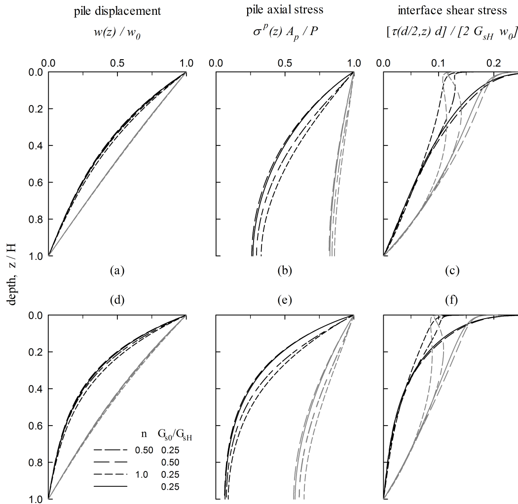
FIGURE 9 Profiles of pile displacement, normal pile axial stresses and shear stresses at the pile-soil interface with depth for two selected geometries of piles embedded in soils with different degrees of inhomogeneity (i.e., n and b from Equations 1 and 2). The black curves refer to E_p/E_{sH} = 100 and the grey curves to E_p/E_{sH} = 1000 . Sub-figures (a) – (c) correspond to L/d = 25 and sub-figures (d) – (f) to L/d = 50 . Number of modes used N = 1500 .
