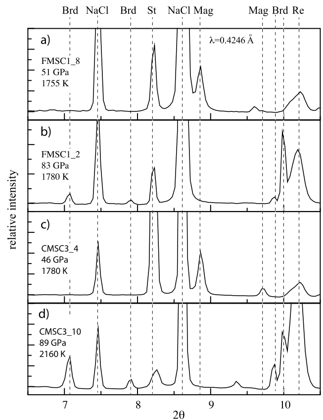
Fig. 3. Selected X-ray diffraction patterns showing relative intensity versus scattering angle 2\theta for P – T quenched run products in the CMSC and FMSC systems (see Table S1). The diffraction lines are labelled according to identified phases; Brd = bridgmanite, St = stishovite, Mag = magnesite as well as the NaCl pressure medium and Re gasket.
