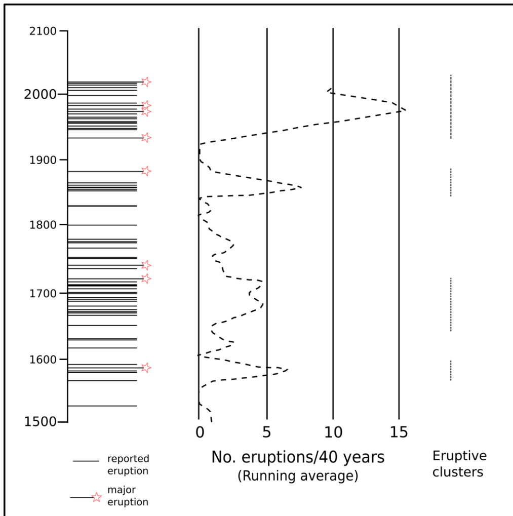
Figure 2: Historic activity of Fuego since 1524. Modified from Rose et al. (1978) via Vallance et al. (2001) and GVP (2018). Four eruptive clusters of 20 – 70 years have defined the eruptive history of Fuego since 1524. Significant eruptions in 1581-2, 1717, 1737, 1880, 1932, 1971, 1974, 1999 and 2018 have been highlighted by red stars.
