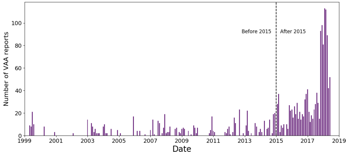
Figure 9: Evidence for new cycle of activity illustrated by number of monthly ash advisory reports generated by Washington VAAC between January 1999 and June 2018. Dashed line indicates boundary between period of moderate activity 1999 – 2014 and period of elevated activity beginning January 2015.
