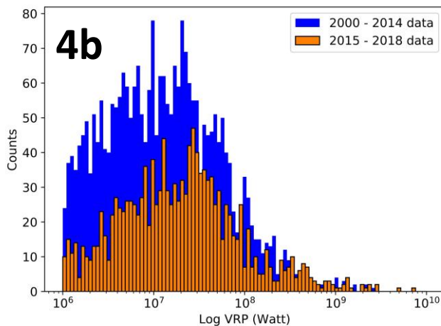
Figure 4a (above): rank-order plot for night-time MIROVA values of Fuego between January 2000 and June 2018 ( n = 4412 ). Figure 4b (below): histogram of two population groups (2000 – 2014 in blue, 2015 – 2018 in orange). Greater number of large VRP values in 2015 – 2018 dataset illustrated by skew of data towards the right of the plot. Figure specifications: single column (3a and 3b vertically stacked), colour
