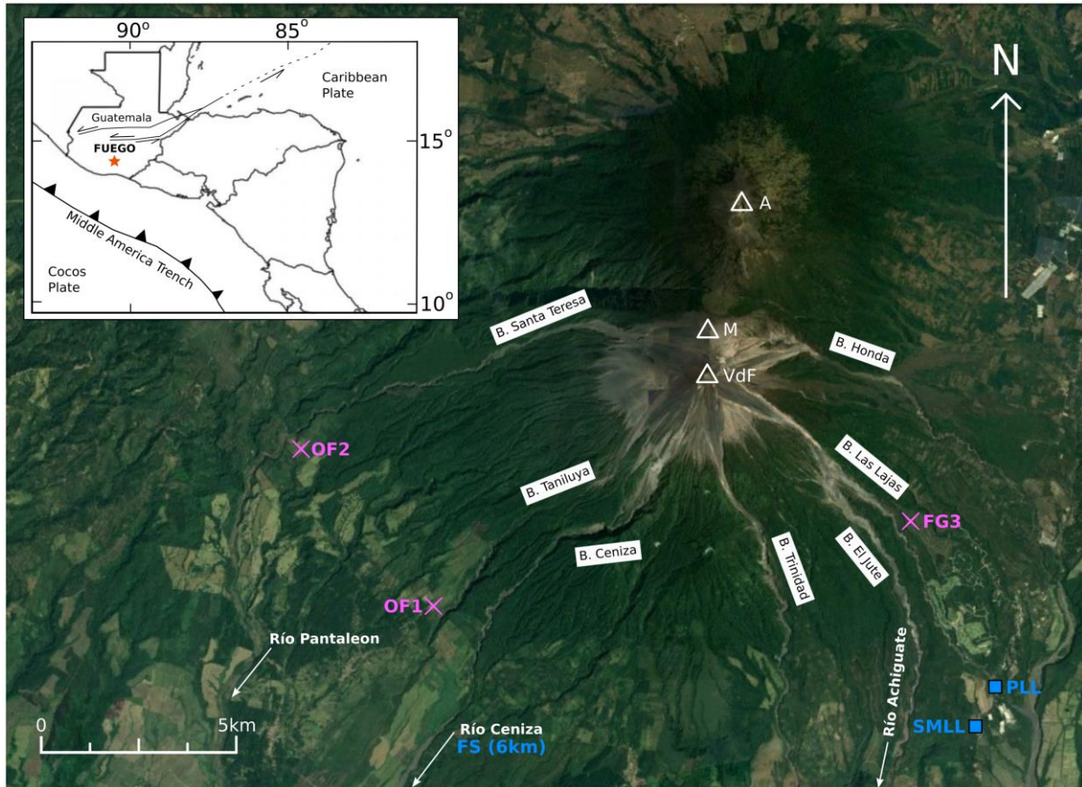
Figure 1: Map of Volcán de Fuego including its seven barrancas (drainage ravines) and major ríos (rivers), with (inset) location of Fuego within Guatemala. Barrancas of Fuego control movement of lava flows, pyroclastic flows, and lahars. Principal eruptive centres of the Fuego-Acatenango massif are (north to south) Volcán Acatenango (indicated as A), La Meseta (M) and Volcán de Fuego (VdF). INSIVUMEH’s two Fuego observatories, OVFGO1 and OVFGO2, are located respectively in the villages of Panimaché Uno and Sangre de Cristo and are indicated by pink crosses. They are labelled as “OF1” and “OF2”. INSIVUMEH’s short-wave seismometer, that provided RSAM data in Section 4, is labelled as “FG3” and indicated by a pink cross. Blue labels indicate the community of San Miguel Los Lotes (SMLL), the Las Lajas bridge (PLL), and the Scout encampment (FS), located approximately 6 km south of map’s southern extent down Barranca Ceniza. Map data: Google, Digital Globe (2018).
