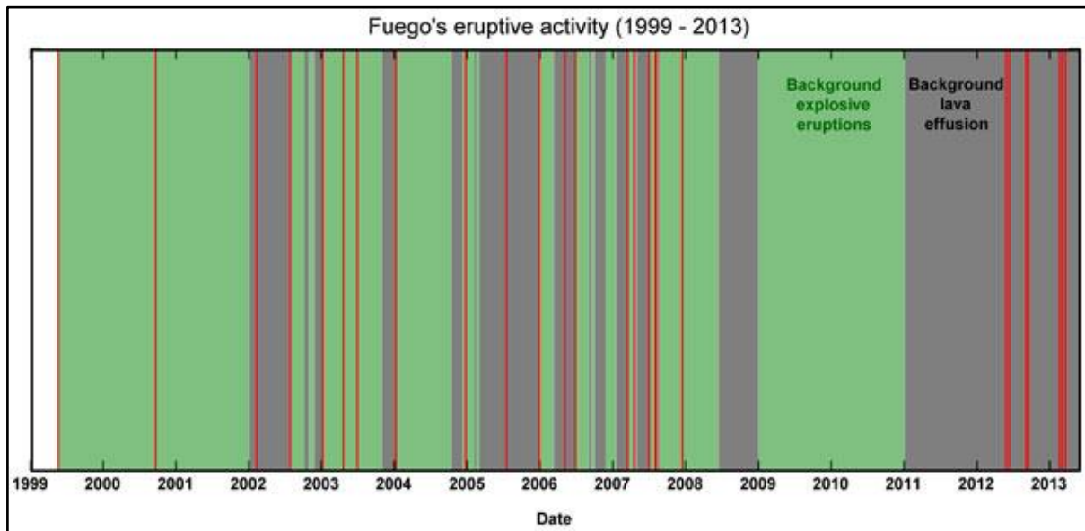
Figure 3: Time-series illustrating activity of Fuego between 1999 and 2013, with colour bars representing different eruption styles. Activity in early 2000s and 2009 – 2011 was dominated by background explosive eruptions (green), while background effusive activity dominated between 2005 – 2007 and 2011 – 2013 (grey). Episodes of significantly above-background explosive activity (paroxysms) illustrated in red. From GVP (2018), originally created by Rüdiger Escobar-Wolf. Figure specifications: 2-column
