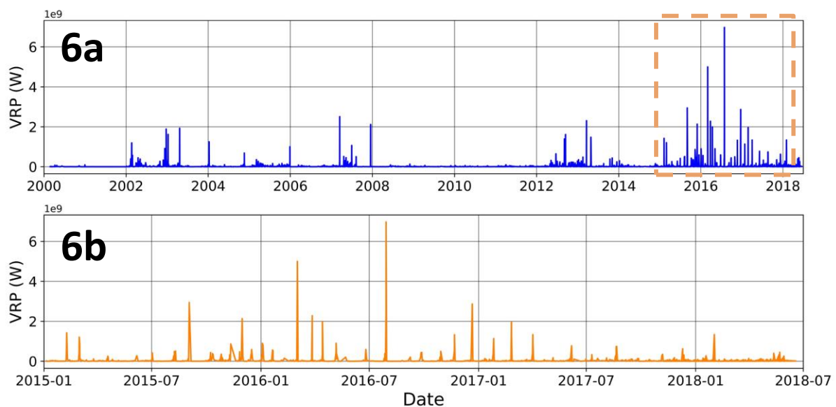
Figure 6a (above): Night-time VRP values from MIROVA track changes in activity at Volcán de Fuego throughout the period 2000 - 2018. Occasional peaks coincide with paroxysmal eruptions as recorded by INSIVUMEH (see Chapter 2). Figure 6b (below): Marked increase in the frequency of large-magnitude VRP values occurs in 2015, with appearance of first short-lived thermal radiation peak on January 5 th , 2015.
