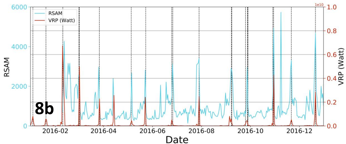
Figure 8a: (Above) Plot of MIROVA values January 2015 – June 2018; y-axis is between 10^6 and 10^{10} W, to filter out low values associated with high angles or adverse viewing conditions. Vertical black lines show timings of all paroxysmal eruptions between 2015 – 2018 identified by INSIVUMEH through special bulletins. Figure 8b: (Below) a subset of above plot, showing time-series of daily RSAM values (blue) against VRP values (red) derived from FG3 measurements. Timings of paroxysmal eruptions reported in INSIVUMEH special bulletins are plotted as dashed lines.
