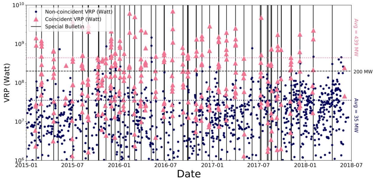
Figure 7: Plot of all night-time VRP values from MIROVA and INSIVUMEH special bulletins between January 2015 and June 2018. Pink triangles represent VRP values coincident ( \pm 48 hours) with INSIVUMEH bulletins (black vertical lines), while blue dots represent VRP values that occur more than 48 hours before/after a special bulletin. Dashed black line represents threshold of 200 MW, above which all paroxysmal eruptions are associated with at least one VRP value. Dotted pink and blue lines represent average of all coincident and non-coincident MIROVA values (439.47 MW and 35.37 MW, respectively).
