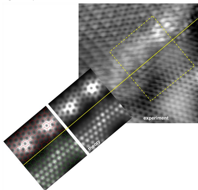
Figure 7: Experimental (on the right) and simulated (in the middle and on the left) STM images for the Pt (111) supported zz -BN/ a -G interface. On the left, the stick model for zz -BN/ a -G interface is superimposed on the simulated STM image. Color coding: h -BN in green, graphene in red. The bias voltage is -1.5 V.
