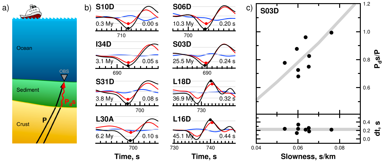
Figure 2. Examples of P_s sediment conversions, and relationship of P_{dS}/P amplitude ratio and delay time ( P_{dS}-P , dt ) with respect to slowness. (a) Schematic of the raypaths of the P wave and P -to- S conversion from the base of the sediment layer, black and red arrows, respectively. (b) Black and red waveforms show the direct P wave and the converted S wave on the vertical and radial component, respectively. Note that there is no incoming signal on the transverse component (blue seismogram). The maximum absolute amplitude of the P phase and the following S phase are marked with dots. The seafloor age and delay time are indicated in the bottom left and right, respectively. Each frame is the record from a different station for the same teleseismic earthquake. (c) Top: P_{dS}/P amplitude ratio with respect to slowness for earthquakes recorded at station S03D. Gray line: P_{dS}/P ratio from synthetic waveforms using a 1-D model and a range of ray parameters. Bottom: Delay time with respect to slowness for earthquakes recorded at station S03D. Horizontal gray line: Average P_s delay time for the station. Note that dt remains stable for a wide range of ray parameters. OBS = ocean bottom seismometer.
