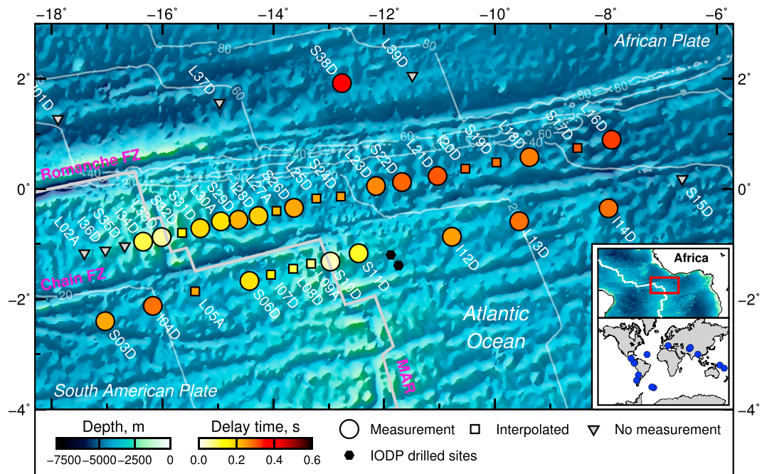
Figure 1. P_s sediment delay time across the Mid-Atlantic Ridge (MAR). Circles are average measurements, squares are linear interpolated measurements from the two nearest neighbors along the same SW-NE profile, and triangles are stations without data, where no interpolation is applied; together they make the Passive Imaging of the Lithosphere-Asthenosphere Boundary seismic network. Black hexagons: International Ocean Drilling Project (IODP) drilled holes Leg 108 sites 662 and 663 (Ruddiman & Janecek, 1989). Thick gray line indicates the ridge (Bird, 2003). Thin contours: Seafloor age at 20-Myr intervals (Müller et al., 2008). Inset maps: Location of the study area (red box) on a regional map and the earthquakes used in this study (blue dots).
