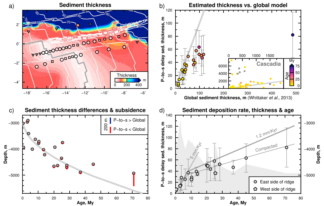
Figure 3. Comparison of estimated sediment thickness with global sediment model, age, subsidence, and production rate. (a) Estimated sediment thickness overlaid on the global sediment model of the world’s oceans (Whittaker et al., 2013). Symbols are the same as in Figure 1. (b) Comparison of P -to- S delay sediment thickness with the global model. Error bars show the uncertainty. Inset: Comparison of estimated sediment thickness with the global model for Cascadia (Rychert et al., 2018). Gray line: One-to-one relationship between the estimated and global model. Different colors represent the seafloor age below the station. Gray dots: Stations without an age constraint. (c) Difference in sediment thickness between estimated and global model (vertical bars), and regional subsidence determined by binning and averaging the acquired bathymetry data (Harmon et al., 2018; depth = 2861 + 324.3 \times \sqrt{age} ). (d) Sediment deposition rate, thickness, and seafloor age. Thick gray line: Estimated accumulated sediment thickness over time at the indicated deposition rates. Thin gray line: Inferred compacted sediment thickness (Alibés et al., 1996). Gray background: The depth at each station. Pentagon and circles: Stations located on west and east side of the ridge, respectively.
