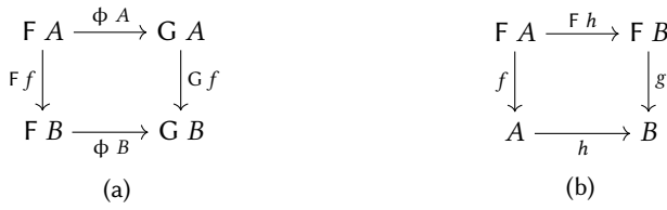
Fig. 1. (a) natural transformation, (b) algebra homomorphism
