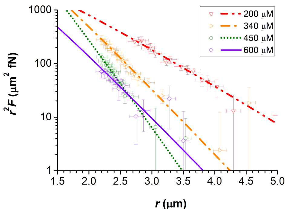
Figure 1. Force profile r^2 F(r) as a function of the centre-to-centre separation r for a pair of PMMA particles in dodecane at n_{\text{salt}} = 200, 340, 450, & 600 \mu\text{M} from blinking optical tweezers measurements. The lines depict fits to Equation (2). The gradient of the line is essentially the (negative) inverse screening length -\kappa . The plot reveals that the measured screening length \kappa^{-1} initially decreases with added salt (as expected), before increasing at 600 \mu\text{M} .
