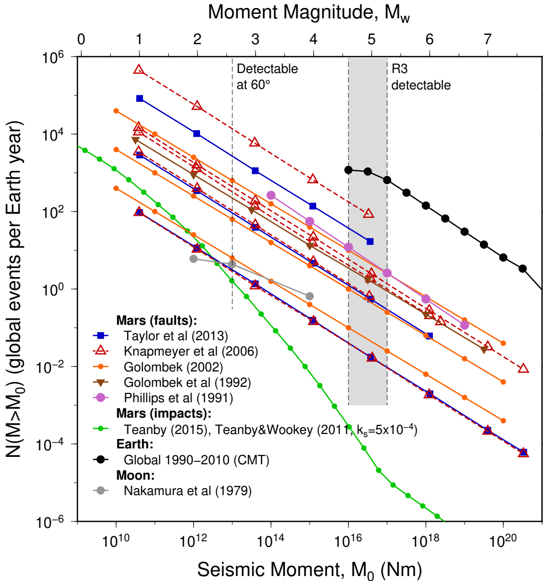
Figure 1: Predictions of martian seismicity in moment release, M_0 versus cumulative number of events in an Earth year for faults and impacts. Mars faulting estimates (see Panning et al. 2017) are based on Phillips (1991), Golombek et al. (1992), Golombek (2002), Knapmeyer et al. (2006) (global) and Taylor et al. (2013) (Cerberus Fossae only). Mars impact seismicity is based on Teanby (2015)'s nominal regional estimates and Teanby and Wookey (2011)'s global estimates with a revised seismic efficiency of k = 5 \times 10^{-4} . For comparison, the seismicity is also shown for the Moon (Nakamura et al. 1979) and Earth (whole globe from Harvard CMT catalogue). The dashed vertical line shows the predicted threshold magnitude for a P wave detection at 60^\circ distance based on the InSight seismometer performance and waveform modeling (Mocquet 1999; Teanby and Wookey 2011). The grey shaded area shows the approximate threshold magnitude and uncertainty for detection of the R3 surface wave (Panning et al. 2015). Both phase arrivals and multiple orbit R1/2/3 energy can be used to determine epicentral distance on Mars.
