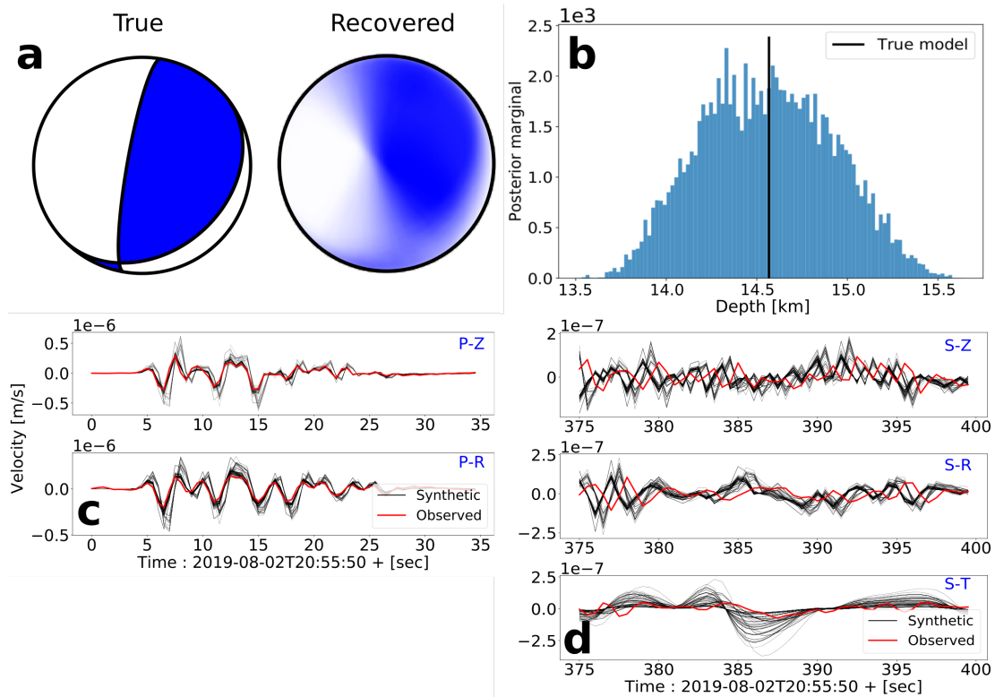
Figure 4: Result of a probabilistic inversion for focal mechanism (strike, dip and rake), depth and epicentral distance for the 2019/08/02 event in the Mars Blind Test dataset. The 'Bayesian Beach Ball' is shown in (a), an overlay of the 1000 best fitting focal mechanisms. (b) shows the depth probability density. While the search was done between 5 and 35 kilometers, the algorithm converged around 14.5 km. (c) shows the waveforms for the 1000 best fitting models. Note that the S-wave fit was generally very low, due to the low amplitude of S-waves in the specific velocity model used for the blind test (d).
