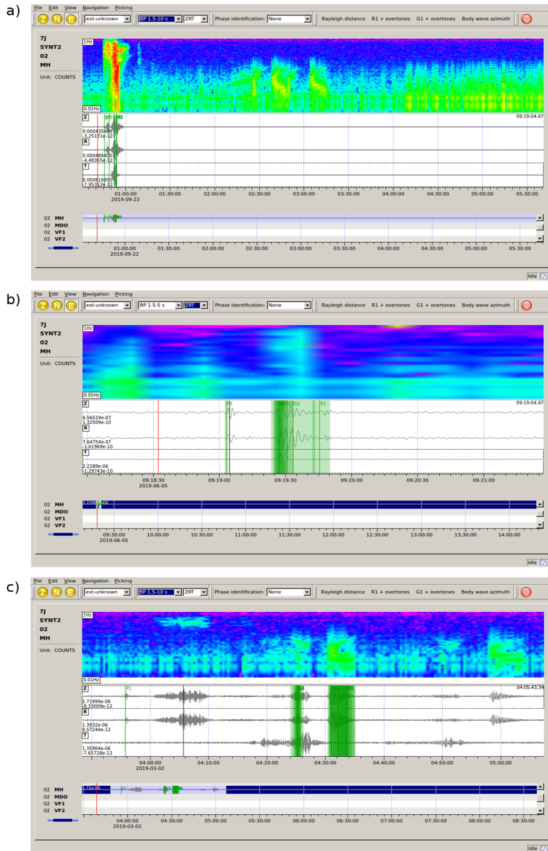
Figure 7: Snapshots from the marslocgui picker window showing waveforms from selected events in the blind test: a) M5.1 at \sim 35^\circ ; b) M2.5 at \sim 3^\circ , and c) M4.3 at \sim 140^\circ . Note the very different time windows. Vertical component spectrograms and 3 component waveforms for the 2sps VBB synthetics are shown at the top and middle respectively. On the bottom are all available channels which includes SP, VBB mass position, weather and housekeeping data as available. On the 3 component VBB waveforms, manual picks for body and surface waves made for each event are indicated by green vertical lines. The estimated origin time is shown on the red line. The first 2 events, the largest teleseism in the catalogue, and a major local event, have very high signal-to-noise and are well located with clear phases - the first event has clear multi-orbit surface waves. The last event is challenging to locate as phase arrivals are emergent and surface waves are weak.
