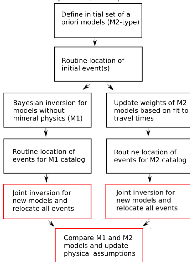
Figure 6: Flowchart of planned procedure for creation of model catalogues and joint updating of structure models and source locations. Boxes in red will only be performed periodically when significant new data become available.
