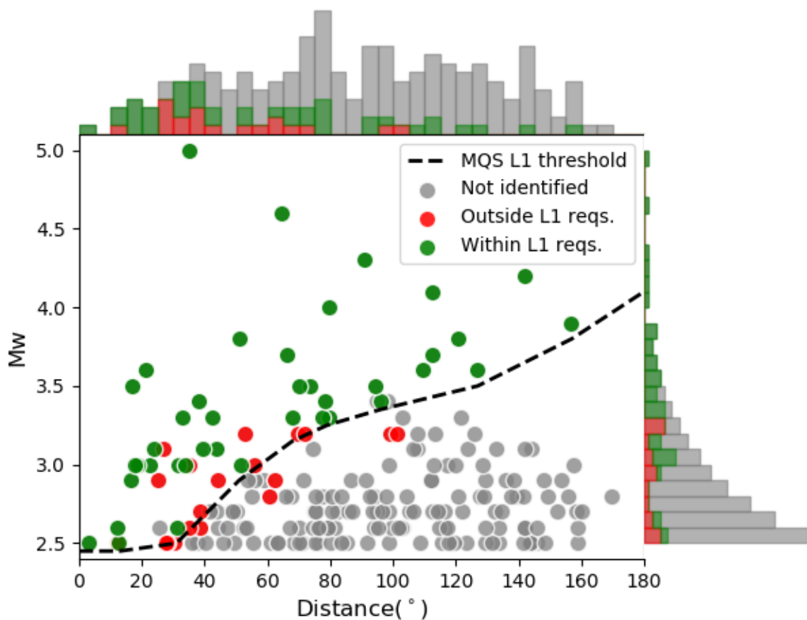
Figure 2: Summary of seismic events included in the MQS Blind Test in terms of magnitude and distance from InSight lander. Events indicated in green and red were detected by MQS, those in grey were not identified (missed). Green events meet the InSight L1 requirements (located well), i.e. the estimated epicentral distances and back azimuths are within \pm 25\% and \pm 20^\circ of the true location. Red events do not meet the L1 requirement (detected only). The black thick dotted line indicates the distance/ magnitude detection threshold of the MQS for the Blind Test. Histograms on the top and right side indicate the proportion of events located well, detected only and missed in terms of magnitude and distance.
