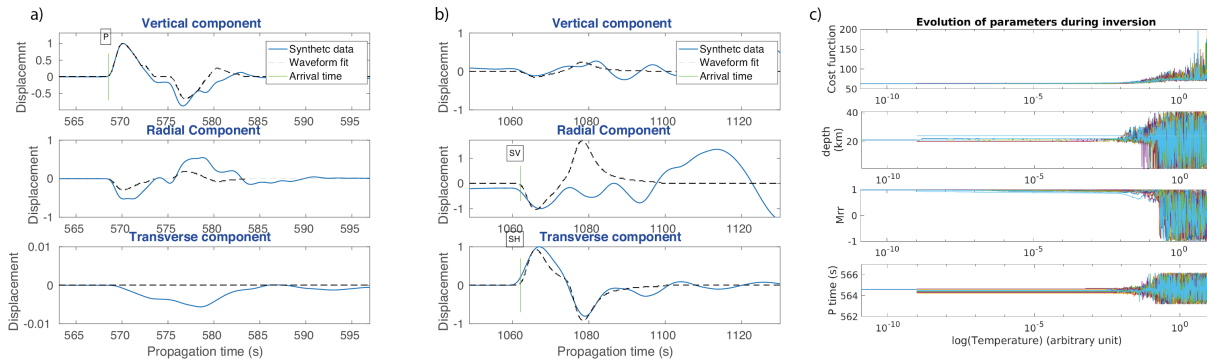
Figure 5: Example SAWIB solution using synthetic seismograms from a Martian event 20 km deep quake at 90° epicentral distance. Fits between observed synthetics and modelled data for the 3-components are shown for the P (a) and SV/SH (b) wave trains. Depth phases are included in the time windows. The evolution of key parameters of the inversion are shown in (c)- from top to bottom: cost function, event depth, one scaled component of moment tensor and P arrival time - as a function of simulated annealing temperature. Colors represent different inversion runs.
