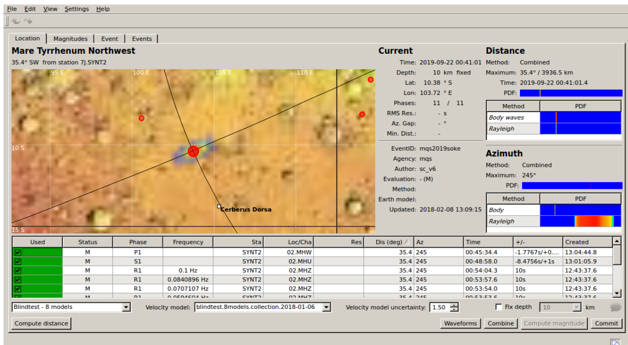
Figure 8: Snapshot of the location summary from the marslocgui location tab for a M5.4 event from the Blind Test. The map shows the currently preferred location as the red dot at the intersection point of the two black lines that indicate preferred distance and back-azimuth. The colours around the epicenter indicate the location PDF. The additional red dots show other events already located in the catalogue. Background image is from Mars Orbiter Laser Altimeter (MOLA; Smith et al. 2001). On the right side of the image are summary PDF information from each method used for this location - the 2 algorithms for distance and azimuth are both used. For the distance, the PDF spans from 0-180°, it is clear both the phase-based ('Body waves') and multiple orbit Rayleigh wave ('Rayleigh') solutions provide very similar distance estimates of about 35°. Some of the phases that are used in the phase-based distance locator (Section 4.2) are shown in the lower table. The model suite used for the phase distance can be selected on the drop-down menu that currently shows 'Blindtest - 8 models'. For the azimuth, the pdf spans from 0-360°. The body wave solution provides 2 peaks, at 65° and 245°(the latter is smaller amplitude so is not clearly visible). The Rayleigh wave back azimuth estimate is far less precise though there is no 180° ambiguity, so when both PDF are combined the correct back azimuth is identified. The PDF in the map is produced by combining the 2 distance and 2 azimuth PDFs.
