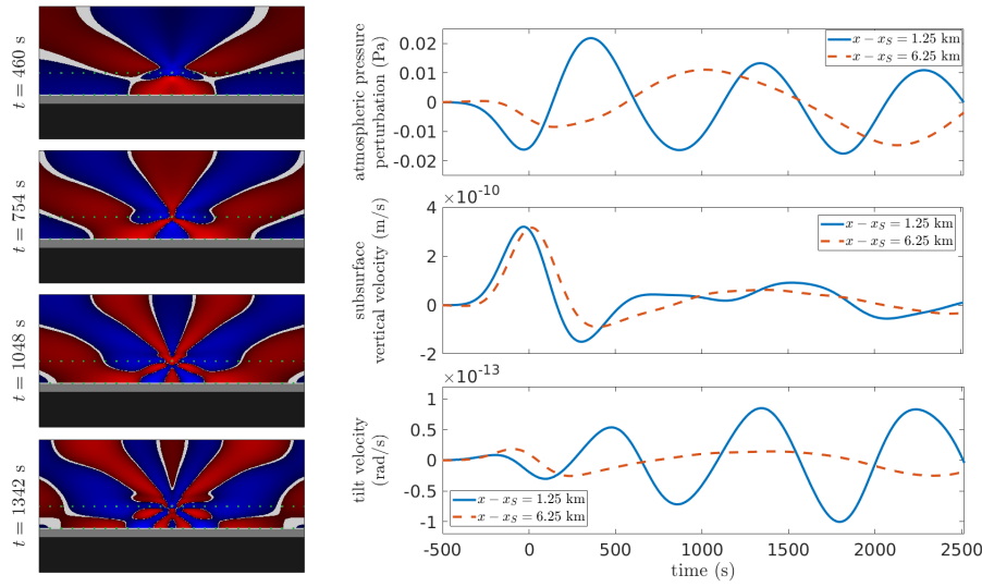
Fig. 15 On the left, from top to bottom, snapshots of pressure perturbations (saturated at 1% of maximum amplitude) at various times during the simulation. Green dots indicate the positions of simulated seismic/infrasounds recording stations, with a separation of 1.25 km in between stations. Bottom part of the snapshots represents the solid viscoelastic model layering. On the right, from top to bottom, pressure variations at the surface (in Pa), ground vertical velocity (in m/s) and rotation speed (in rad/s), along an axis perpendicular to simulated plane, at two stations with horizontal distances from the source of 1.25 km (continuous line) and 6.25 km (dashed line). Note that the snapshots does not show the vibrations in the ground due to their very low amplitude, but they are computed in the simulation.
