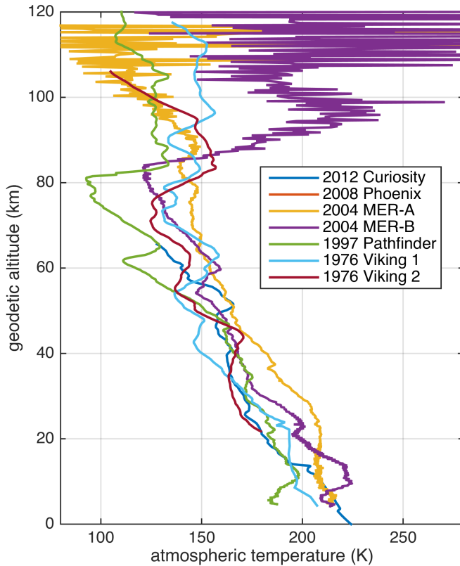
Fig. 14 Profiles of temperature acquired during the Entry Descent and Landing phases of previous Martian missions. References for each profile are listed in the text. Local time and season for each profile (Paton et al. 2018) are as follows: (Viking Lander 1) 16:13 L_s = 97^\circ , (Viking lander 2) 09:49 L_s = 121^\circ , (Pathfinder) 02:56 L_s = 143^\circ , (MER A Spirit) 14:16 L_s = 327^\circ , (MER B Opportunity) 13:13 L_s = 339^\circ , (Phoenix) 16:00 L_s = 77^\circ , (Curiosity) 15:00 L_s = 151^\circ . Those profiles carry information both on the global climate (e.g. planetary waves, seasonal trends) and on regional-to-local processes (e.g. gravity waves, possibly leading to subcondensation temperatures as is the case for the Pathfinder profile).
