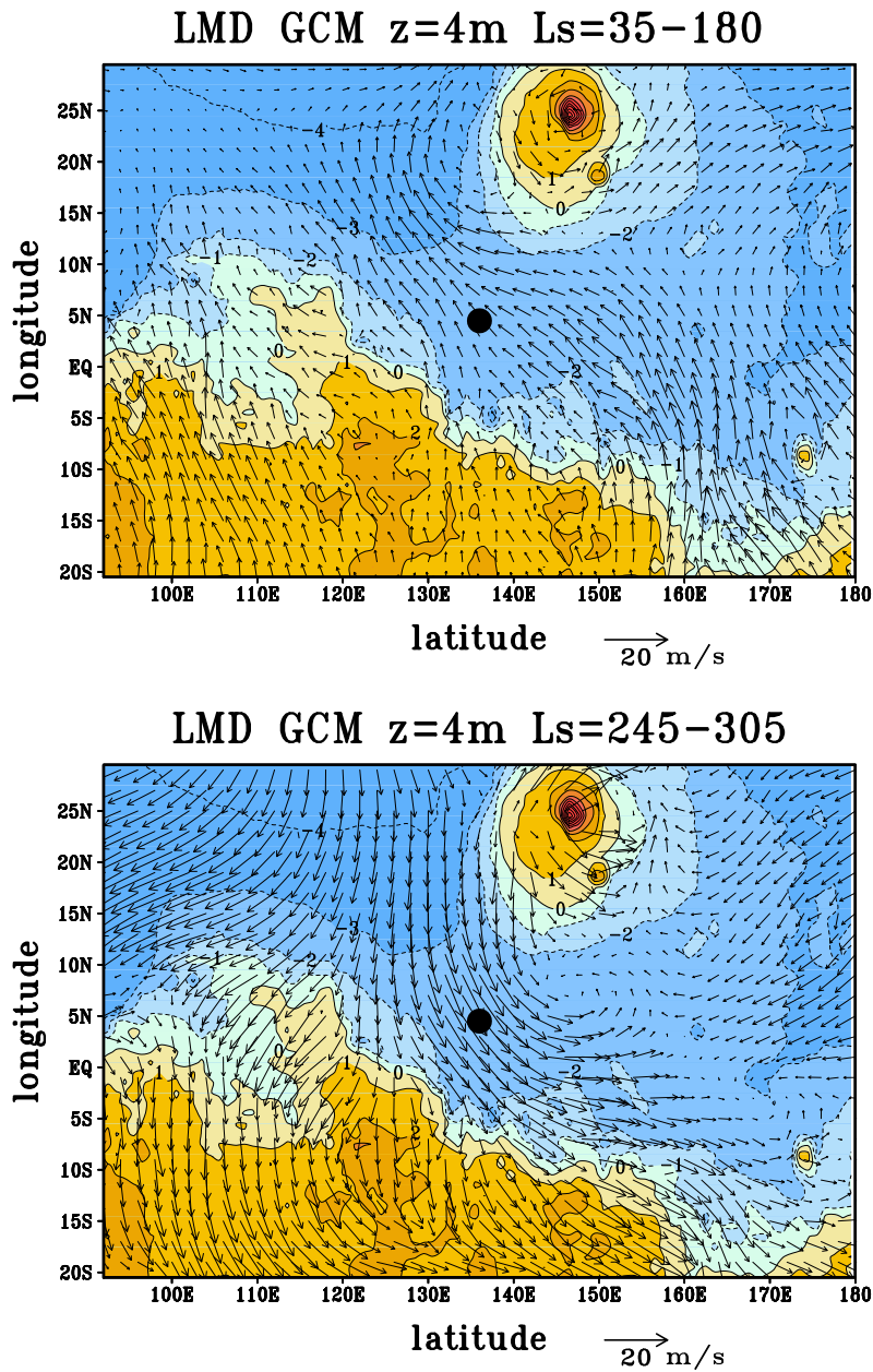
Fig. 9 Mean near-surface winds (at 4 m above ground) in the InSight landing site area as predicted by the LMD Global Climate Model (Forget et al. 1999; Pottier et al. 2017) for two characteristic periods of the atmospheric circulation (regime \mathcal{R}_1 at L_s = 35 - 180^\circ on top panel and regime \mathcal{R}_2 at L_s = 245 - 305^\circ on bottom panel). During those two characteristic periods, the wind direction does not change much over the course of one Martian sol (see Figure 8), hence showing here the diurnal average is meaningful. The black dot illustrates the location of InSight. Color shading shows the underlying topography.
