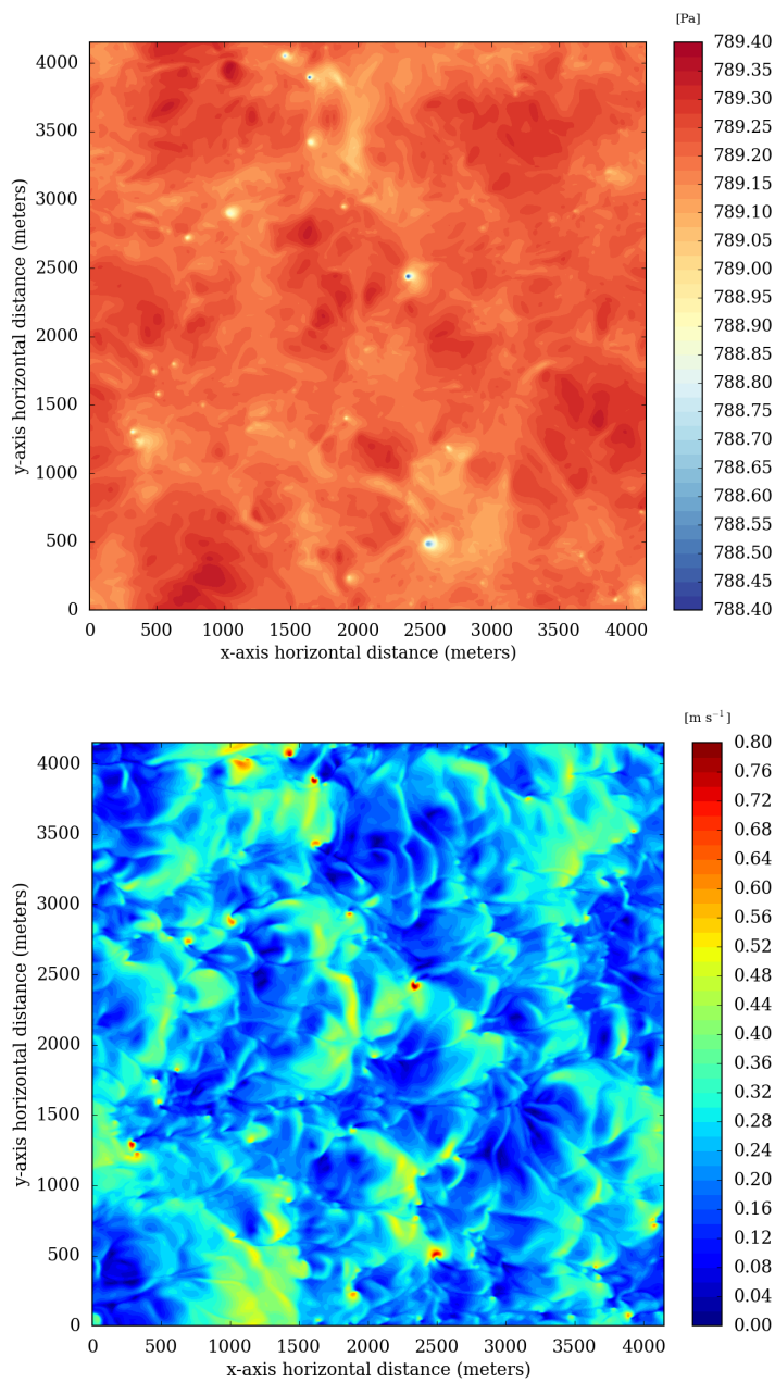
Fig. 11 Horizontal maps of surface pressure (top) and friction velocity (bottom), as predicted by the 10-m resolution turbulence-resolving LES described in the text, based on the model by Spiga et al. (2010). Conditions are close to 9AM local time. The impact of both convective vortices, and gusts associated with convective cells, can be noticed on those maps. Friction velocity is a proxy for near-surface winds (see section 6.1) and their ability to exchange heat and material between the surface and atmosphere.
