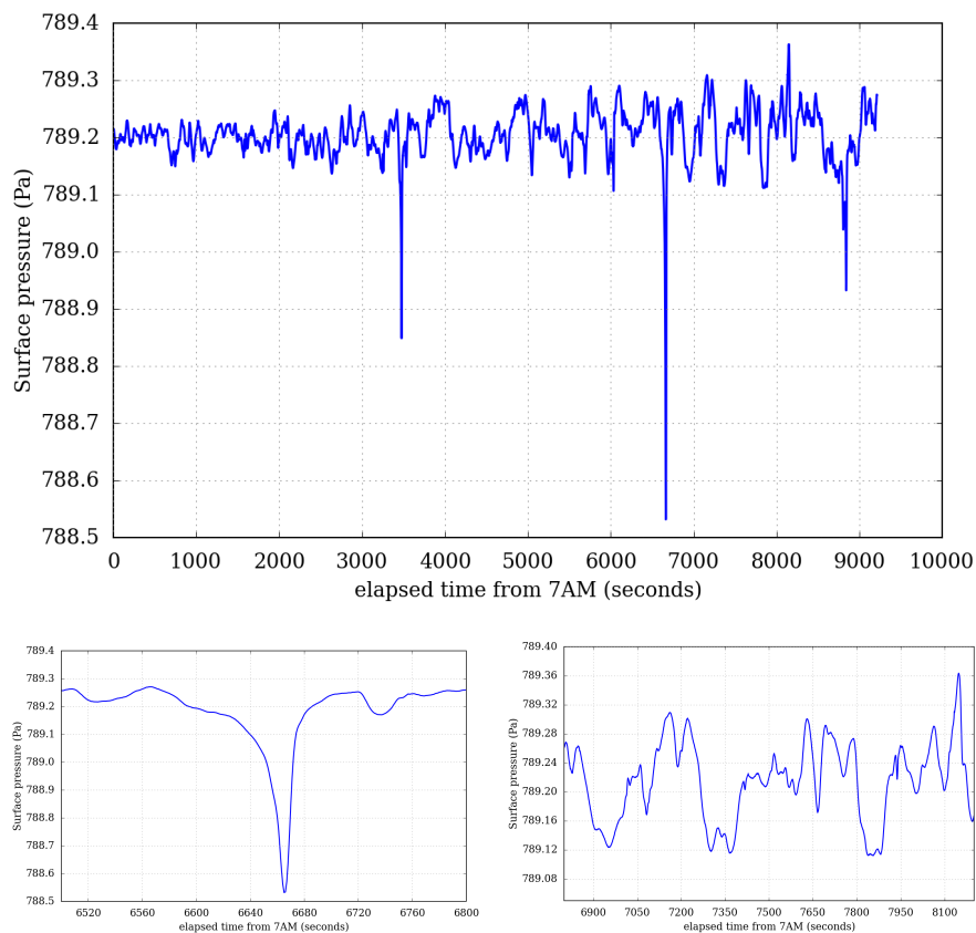
Fig. 12 Temporal 1-Hz series of surface pressure predicted by the 10-m resolution turbulence-resolving LES model. The location corresponds to the central pressure drop in Figure 11. This figure emulates what would be observed by the InSight PS. The two bottom magnified views correspond to the two notable phenomena in the pressure temporal variations: sudden pressure drops corresponding to a passing convective vortex (a “dustless” devil, see e.g. Spiga et al. 2016) and periodic signals corresponding to convective cells advected by the background wind (Spiga 2012).
