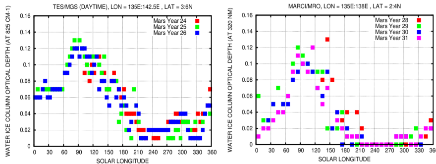
Fig. 5 Seasonal evolution of the water ice clouds observed during daytime above the InSight landing site. Top : Cloud opacity at 12.1 \mu\text{m} ( 825 \text{ cm}^{-1} ) at about 2pm local time as retrieved by Smith (2004) from the MGS/TES observations. Bottom : Cloud daytime UV opacity at 0.320 \mu\text{m} as retrieved by Wolff et al. (2014) from the MRO/MARCI observations. Assuming simple spherical shapes for water ice particles with effective radius 3 microns, the TES opacity at 12.1 \mu\text{m} can be converted to the MARCI opacity at 0.320 \mu\text{m} by multiplying by a factor \sim 1.86 [ 1.37 to account for the absorption (TES) vs. extinction (MARCI) difference (Wolff and Clancy 2003) and 1.36 to account for the wavelength difference (Clancy et al. 2003)]. Note that water ice opacity has also been retrieved from several other instruments (e.g. THEMIS, PFS): only TES and MARCI results are shown here for the sake of simplicity.
