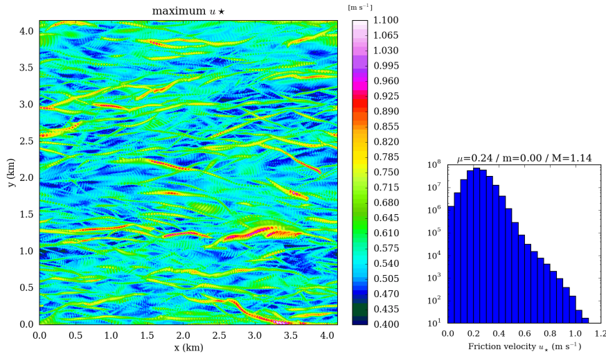
Fig. 13 Results predicted by the 10-m resolution turbulence-resolving LES model. The horizontal map corresponds to the maximum values of friction velocity for each grid point over the 2.5 hours of simulated hours. The areas of high friction velocity correspond to the passage of convective vortices, and would be representative of dust devil tracks shall dust could be mobilized from the surface of Mars in this area. Relatively large friction velocity are also noticed as a result of passing convective cells in the scene. The histogram corresponds to the mapped values: friction velocity associated with turbulence could well exceed the mean value associated with the background wind (Fenton and Michaels 2010; Mulholland et al. 2015; Nishizawa et al. 2016).
