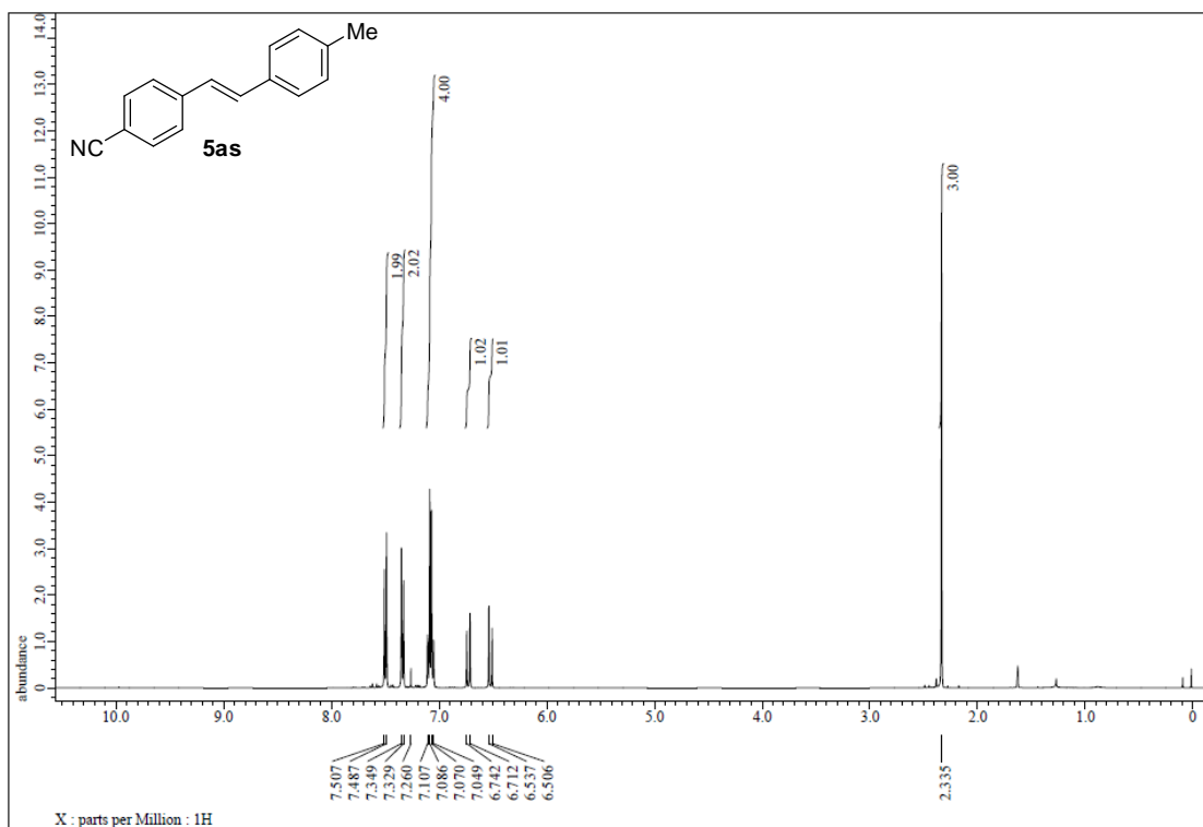
Figure S201. 1 H NMR spectrum of 5as, related to Figure 5.
