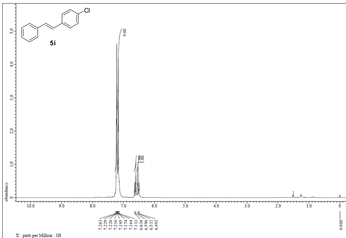
Figure S123. 1 H NMR spectrum of 5i , related to Figure 4.
