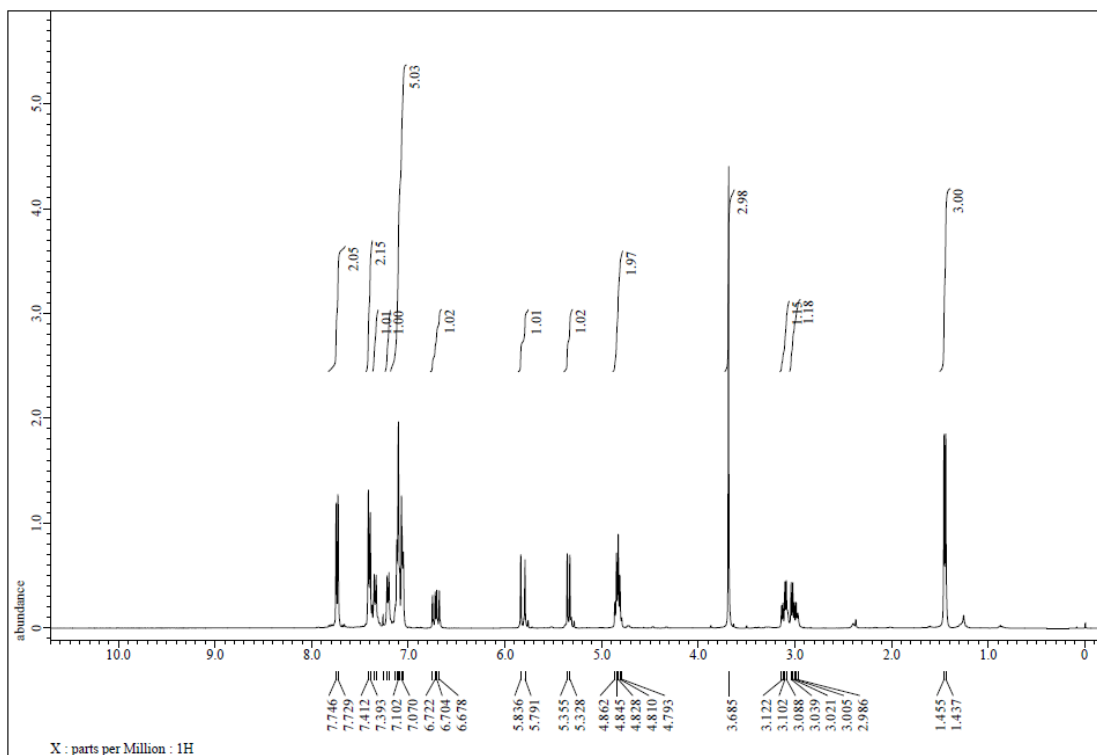
Figure S42. 1 H NMR spectrum of 3t, related to Figure 2.
