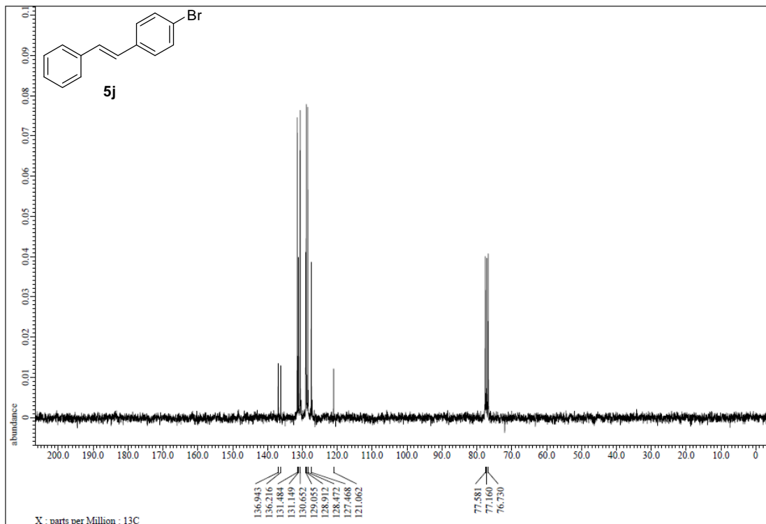
Figure S126. 13 C NMR spectrum of 5j, related to Figure 4.
