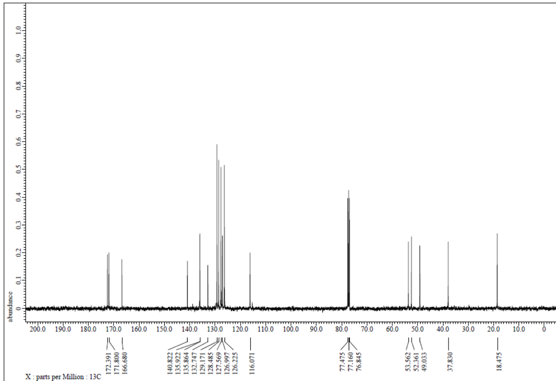
Figure S43. 13 C NMR spectrum of 3t, related to Figure 2.
