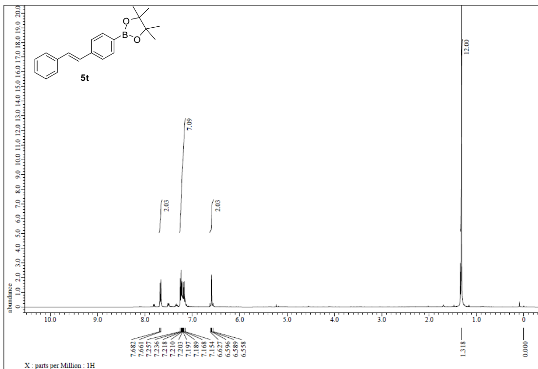
Figure S147. 1 H NMR spectrum of 5t, related to Figure 4.
