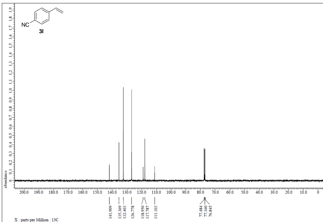
Figure S27. 13 C NMR spectrum of 3l, related to Figure 2.
