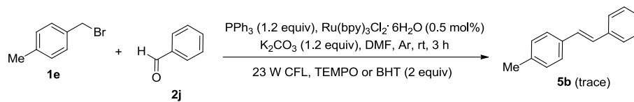
Figure S236 | Reaction of 1e with 2j in the presence of TEMPO or BHT, related to Figure 1.
