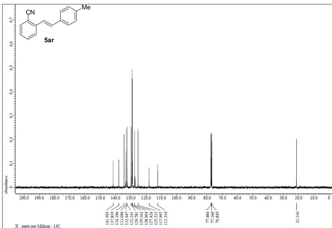
Figure S200. 13 C NMR spectrum of 5ar, related to Figure 5.
