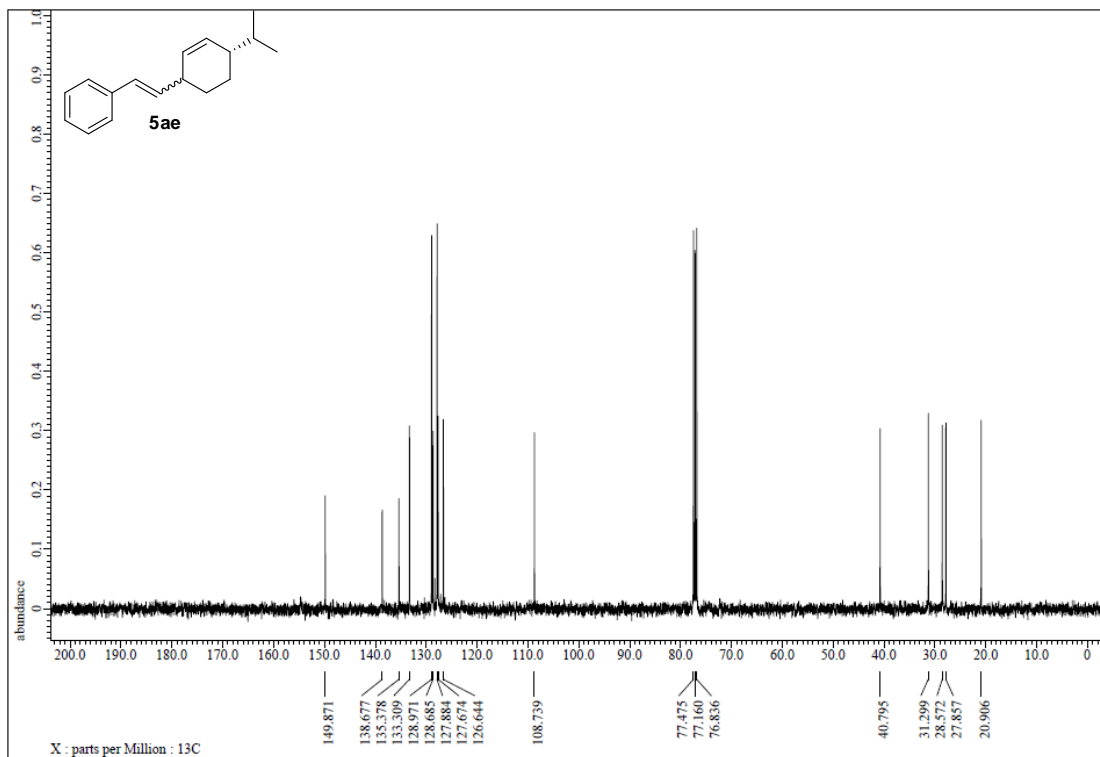
Figure S171. 13 C NMR spectrum of 5ae, related to Figure 4.
