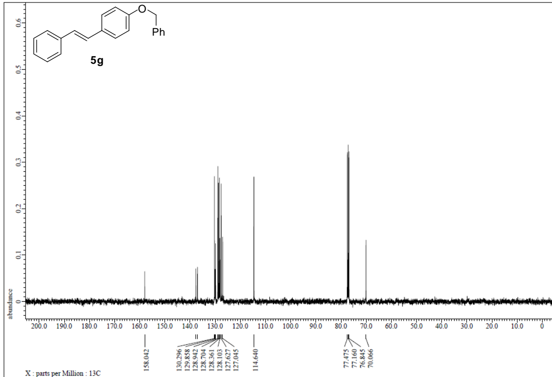
Figure S120. ^{13}\text{C} NMR spectrum of 5g, related to Figure 4.
