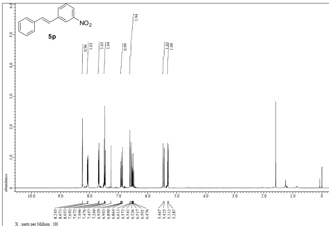
Figure S139. 1 H NMR spectrum of 5p, related to Figure 4.
