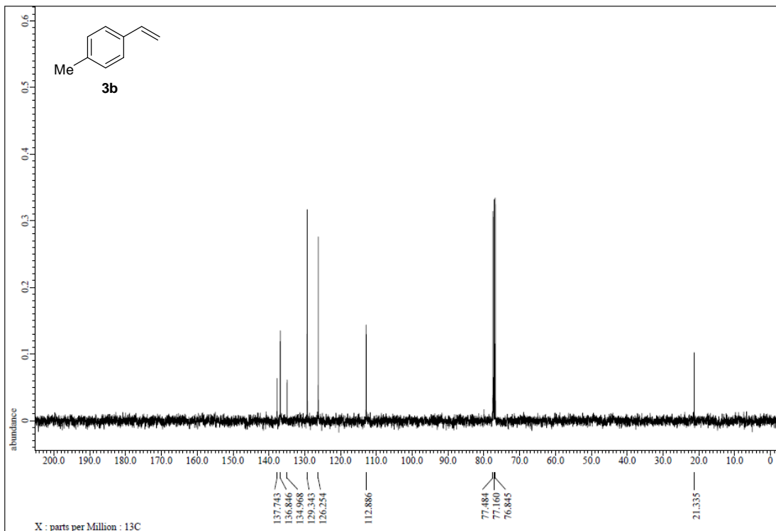
Figure S4. 13 C NMR spectrum of 3b, related to Figure 2.
