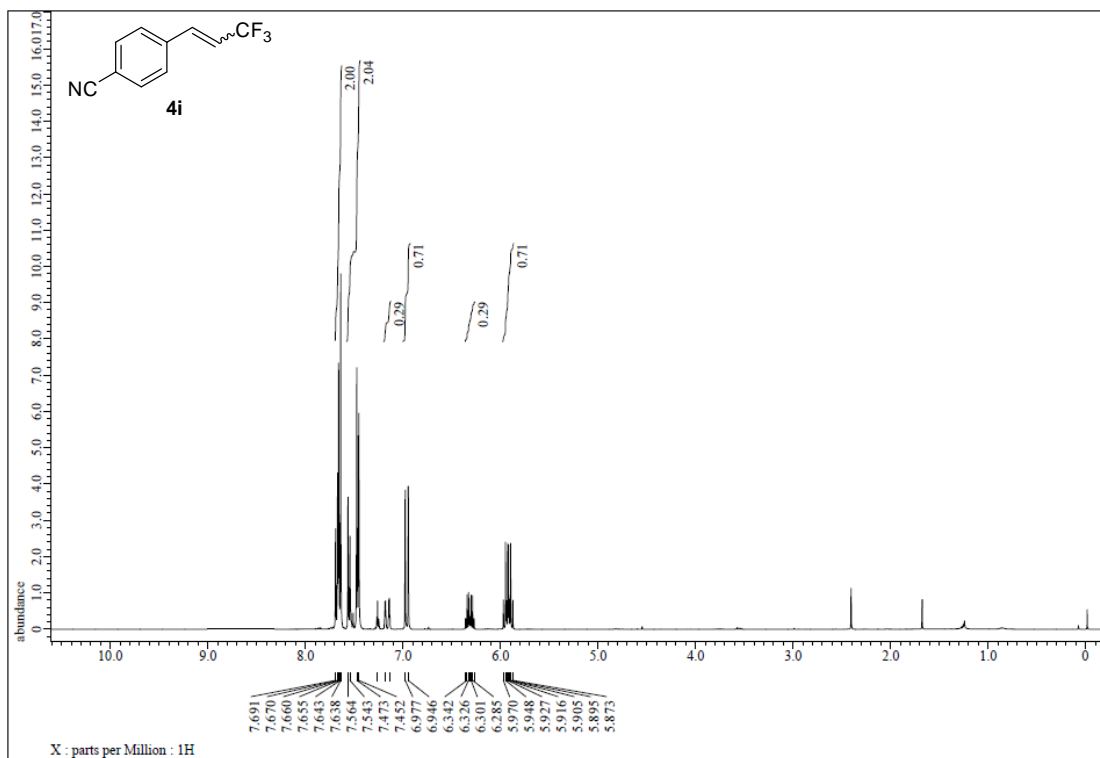
Figure S86. 1 H NMR spectrum of 4i, related to Figure 3.
