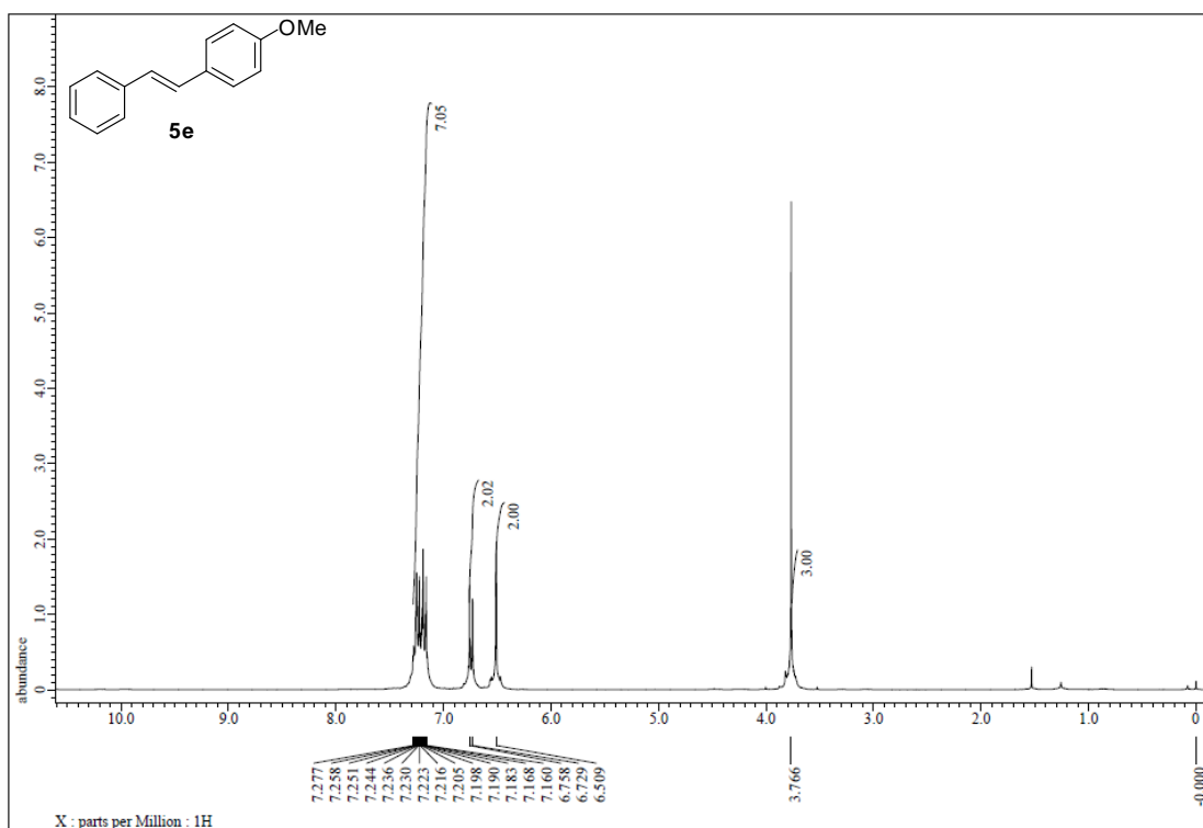
Figure S115. 1 H NMR spectrum of 5e, related to Figure 4.
