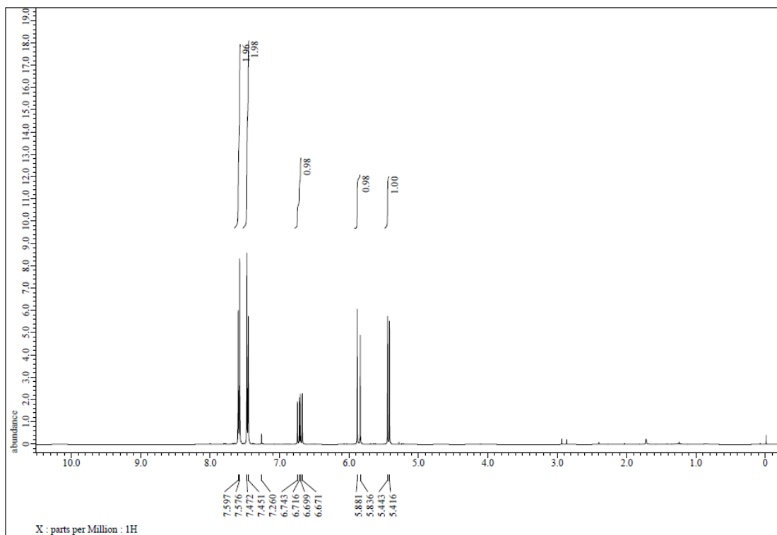
Figure S26. 1 H NMR spectrum of 3l, related to Figure 2.
