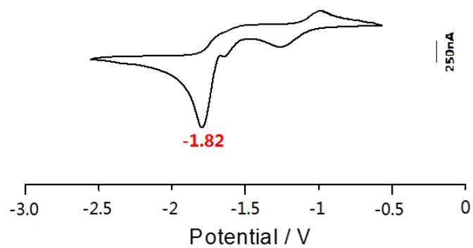
Figure S237. The CV of p -Tolualdehyde (0.1M) in 0.1M nBu 4 NPF 6 in DMF at a Pt working electrode with a Pt counter electrode and Ag wire quasireference, related to Figure 1. Potential sweep rate was 50 mV/s.
