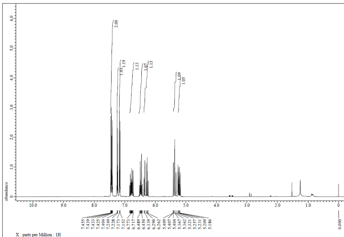
Figure S50. 1 H NMR spectrum of 3x, related to Figure 2.
