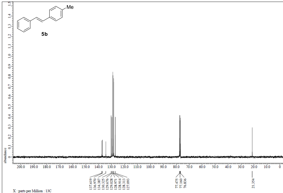
Figure S110. ^{13}\text{C} NMR spectrum of 5b, related to Figure 4.
