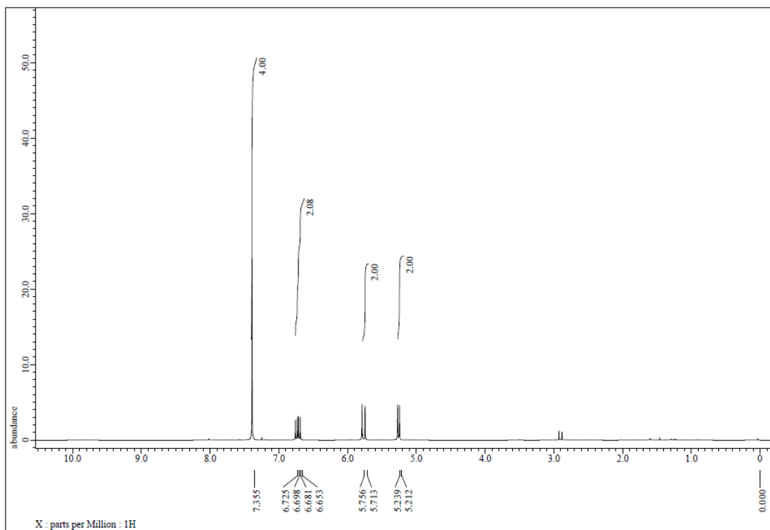
Figure S34. ^1\text{H} NMR spectrum of 3p, related to Figure 2.
