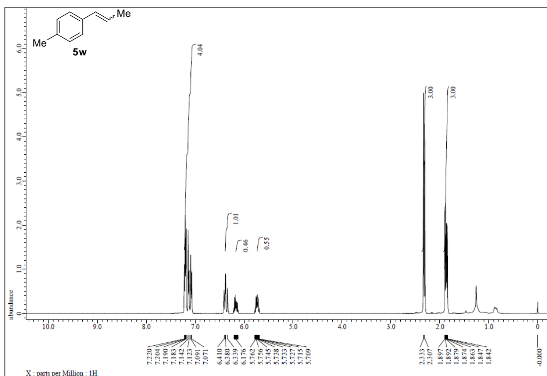
Figure S154. 1 H NMR spectrum of 5w, related to Figure 4.
