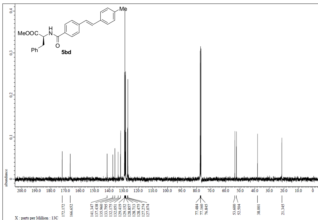
Figure S224. 13 C NMR spectrum of 5bd, related to Figure 5.
