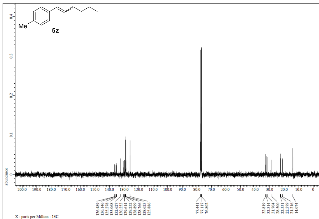
Figure S161. 13 C NMR spectrum of 5z, related to Figure 4.
