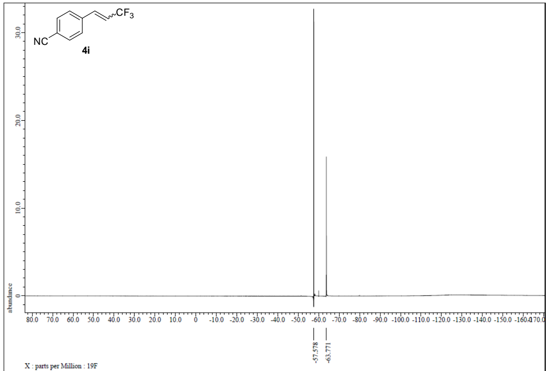
Figure S88. 19 F NMR spectrum of 4i , related to Figure 3.
