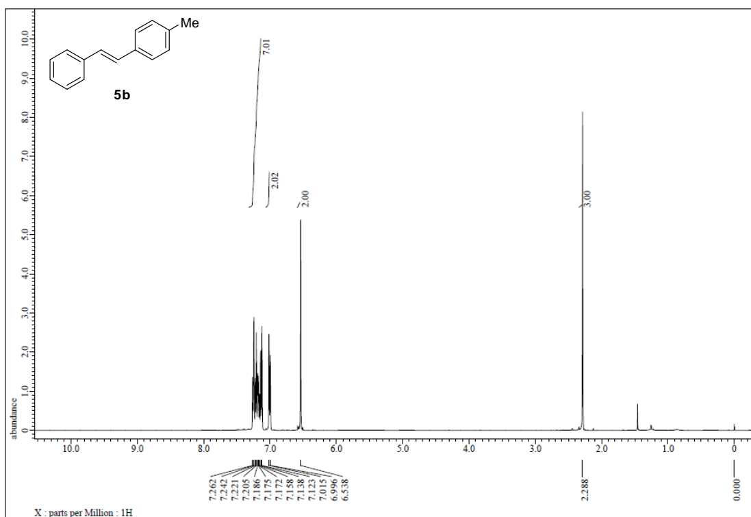
Figure S109. ^1\text{H} NMR spectrum of 5b, related to Figure 4.
