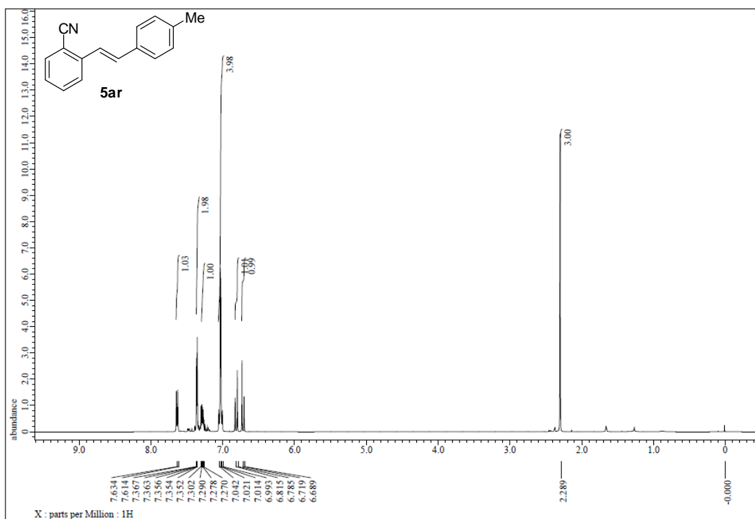
Figure S199. 1 H NMR spectrum of 5ar, related to Figure 5.
