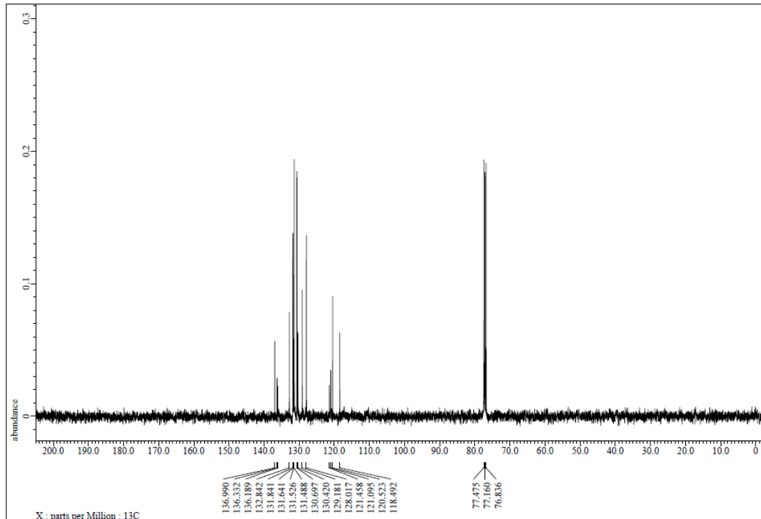
Figure S51. 13 C NMR spectrum of 3x, related to Figure 2.
