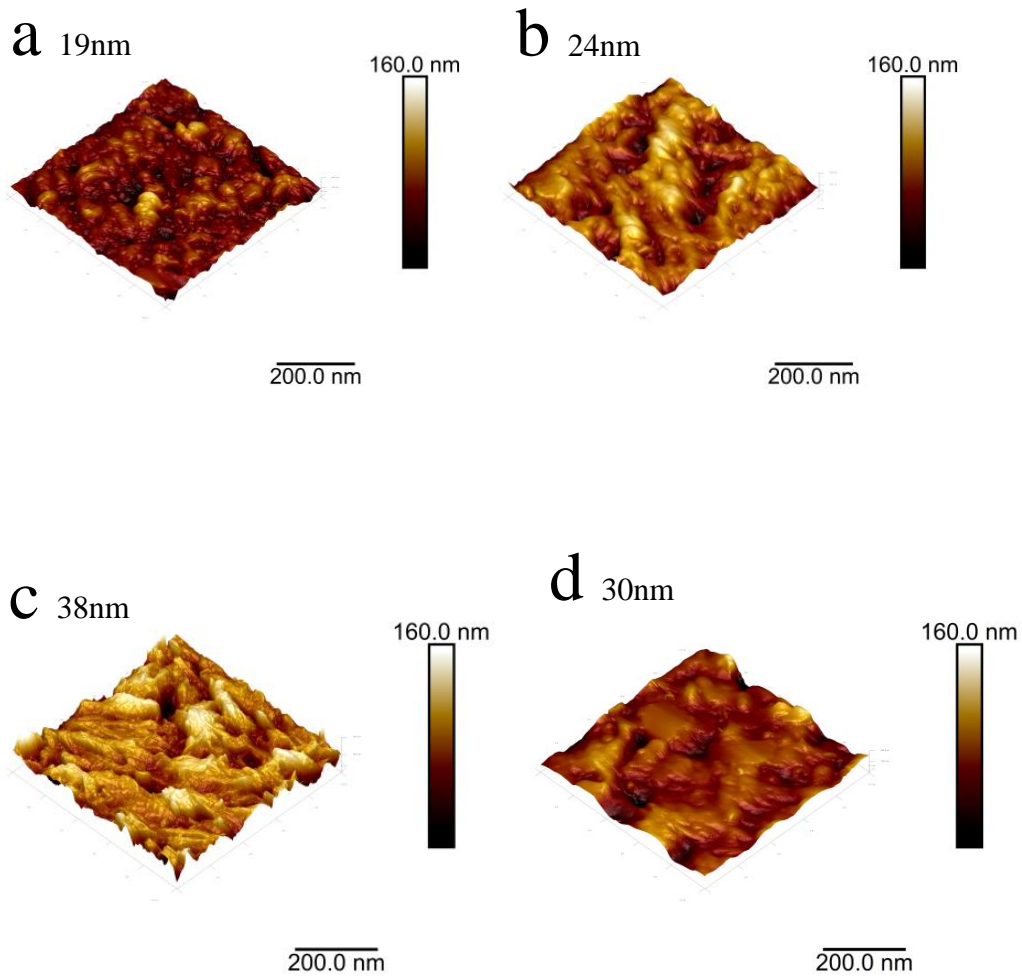
Figure 7. AFM characterization and average surface roughness (nm) for a 1 \mu\text{m} \times 1 \mu\text{m} area of (a) a pure cellulose fiber (b) a Li:Cell 25:75 fiber (c) a Li:Cell 50:50 fiber and (d) a Li:Cell 75:25 fiber. Root mean square (RMS) roughness' of the fibers' surfaces are stated in the insets of the images.
