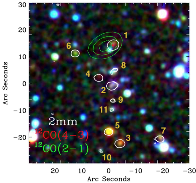
Figure 4. False-color image of the core of our protocluster at z_{\text{spec}} = 4.002 , obtained from our I , K_S -band and IRAC imaging. The positions of the 11 DRC components are highlighted by white contours; ^{12}\text{CO}(2-1) emission from ATCA is shown with green contours and the ALMA ^{12}\text{CO}(4-3) emission is shown with red contours (note that this faint emission is on top of DRC-1). All contours run from 4\sigma to 6\sigma in steps of 1\sigma . Most DRC components are detected in at least one optical/near-IR band and a variety of colors is seen, with the brightest sources at 2 mm having the reddest optical/near-IR colors.
