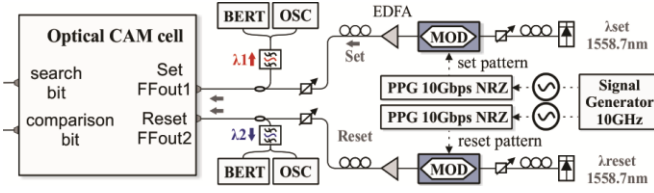
Fig. 4. Experimental setup used for Content Write operation at 10Gb/s
