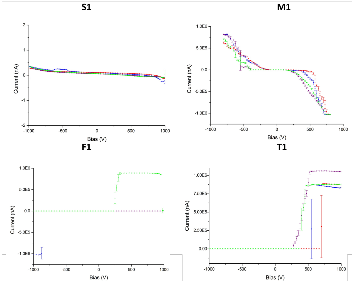
Figure 3. Dark current measurements for the four diamond detector devices.
