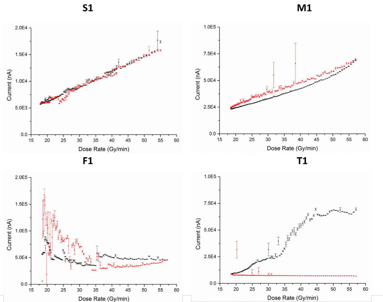
Figure 4. Current versus dose rate for the four diamond devices tested at the Dalton Cumbria Facility.
