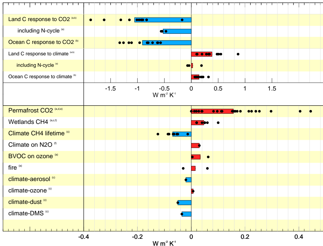
Figure 6.20: A synthesis of the magnitude of biogeochemical feedbacks on climate. Gregory et al. (2009) proposed a framework for expressing non-climate feedbacks in common units ( \text{W m}^{-2} \text{K}^{-1} ) with physical feedbacks, and Arneth et al. (2010) extended this beyond carbon cycle feedbacks to other terrestrial biogeochemical feedbacks. The figure shows the results compiled by Arneth et al. (2010), with ocean carbon feedbacks from the C4MIP coupled climate-carbon models used for AR4 also added. Some further biogeochemical feedbacks are also shown but this list is not exhaustive. Black dots represent single estimates, and coloured bars denote the simple mean of the dots with no weighting or assessment being made to likelihood of any single estimate. There is low confidence in the magnitude of the feedbacks in the lower portion of the figure, especially for those with few, or only one, dot. The role of nitrogen limitation on terrestrial carbon sinks is also shown — this is not a separate feedback, but rather a modulation to the climate-carbon and concentration-carbon feedbacks. These feedback metrics are also likely to be state or scenario dependent and so cannot always be compared like-for-like (see Section 6.4.2.2). Results have been compiled from (a) Arneth et al. (2010), (b) Friedlingstein et al. (2006), (c) HadGEM2-ES (Collins et al., 2011) simulations, (d) Burke et al. (2012), (e) von Deimling et al. (2012), (f) Stocker et al. (2013). Note the different x-axis scale for the lower portion of the figure.
