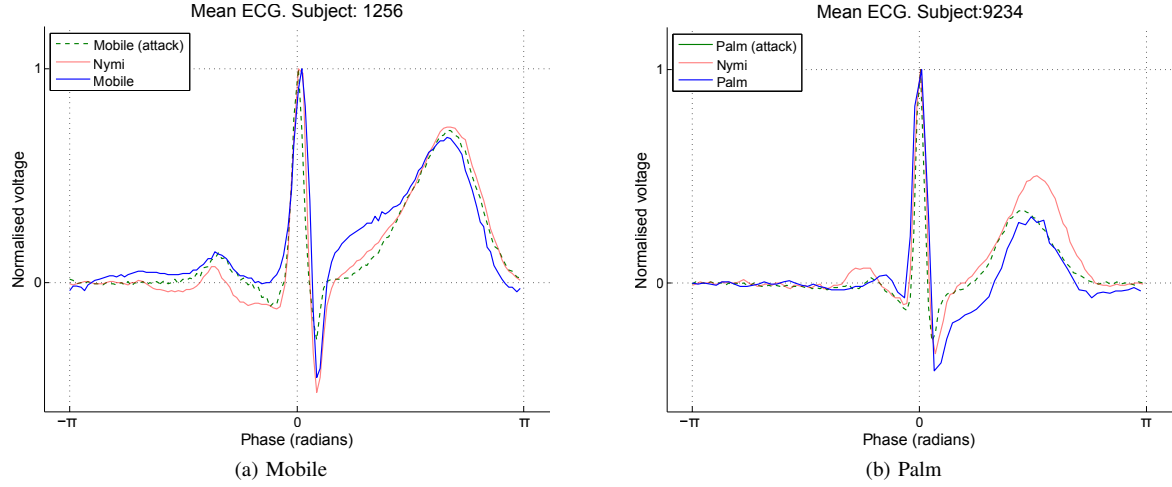
Fig. 13: Comparison of mean ECGs among source signal, corresponding attack signal and target Nymi signal.
