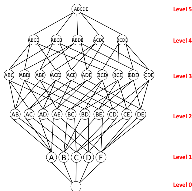
Fig. 2 Complete lattice for a product with five parts
